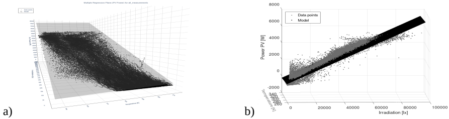
Fig. 5: 3D linear regression model obtained for all data, the dependence of electricity production a) on panel temperature; b) on solar radiation and temperature of panels
