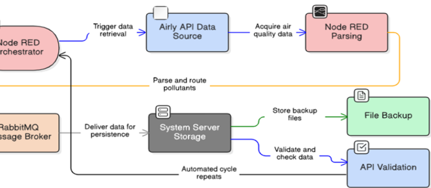
Fig. 2 Data Flow Steps
