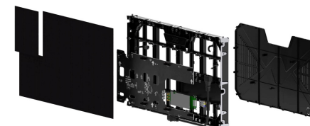
Exploded view · modules, chassis, rear cover
