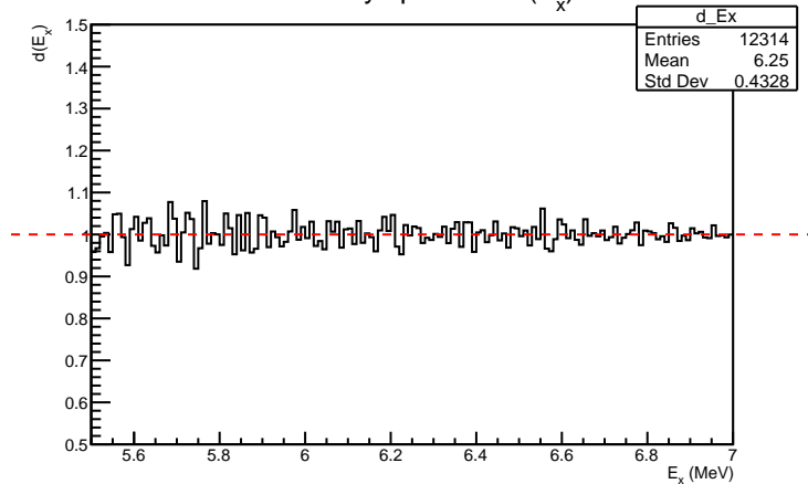
Stationary spectrum d(E_x)
