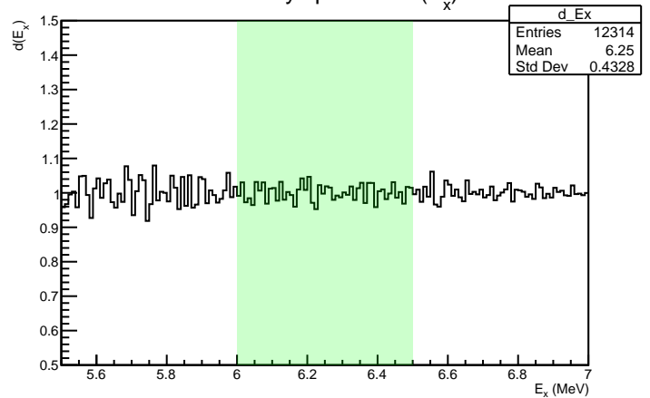
Stationary spectrum d(E_x)
