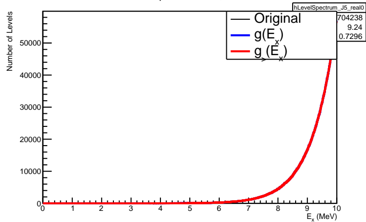
Level Spectrum J=5, Real 0
