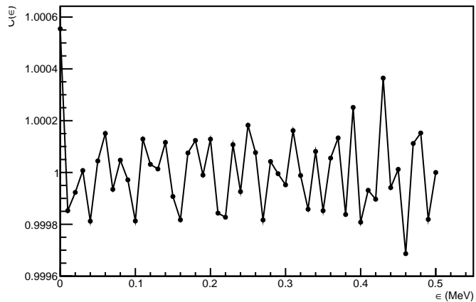
Autocorrelation Function
