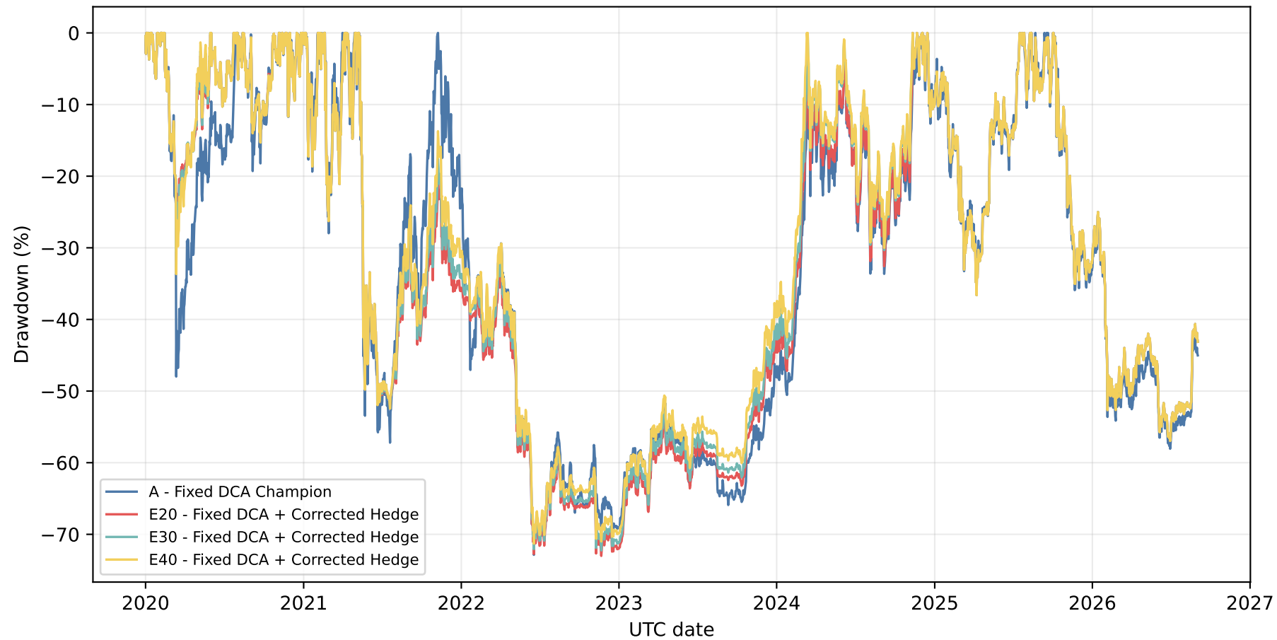
V2 Drawdown Curves
