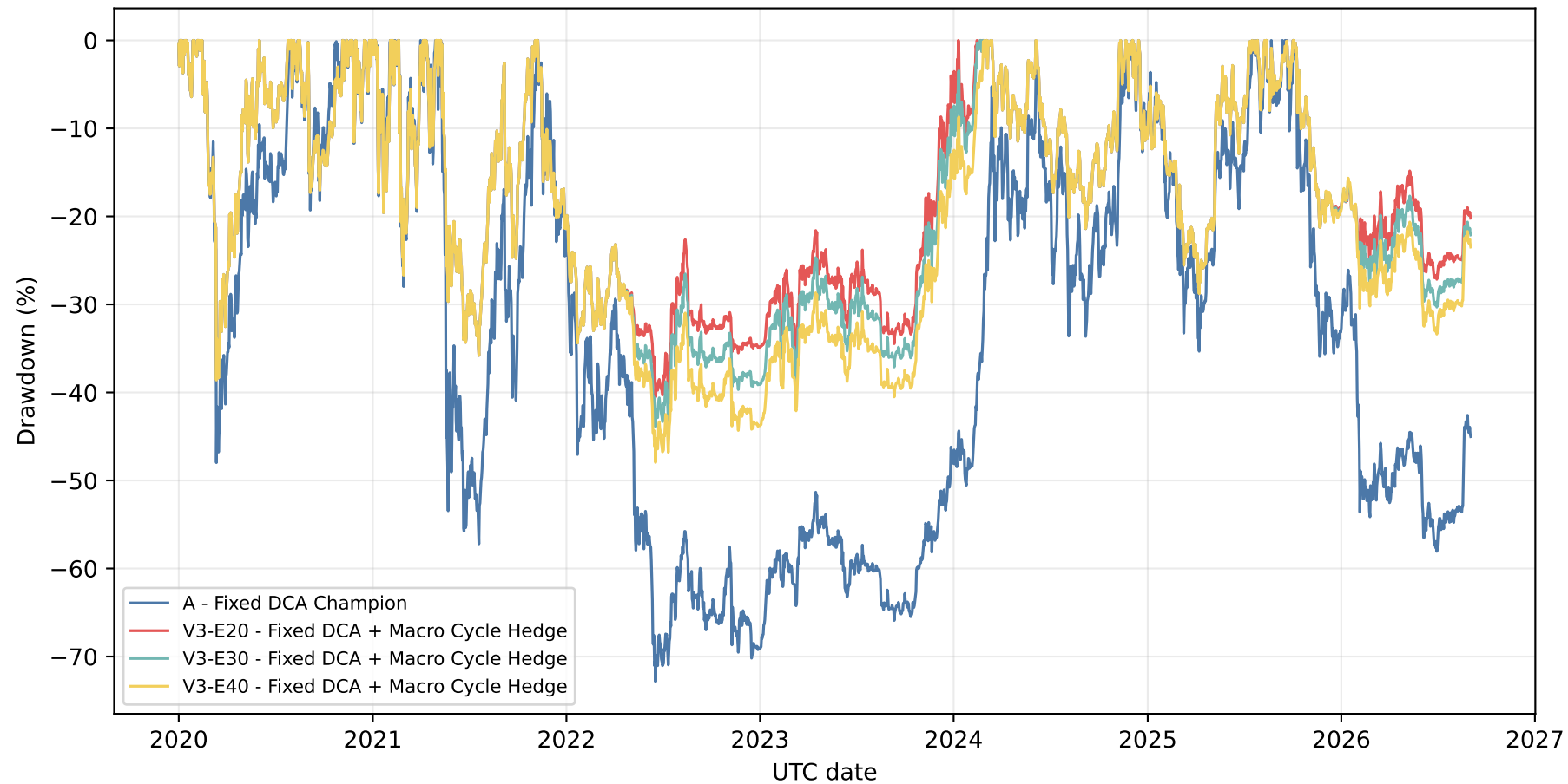
V3 Drawdown Curves
