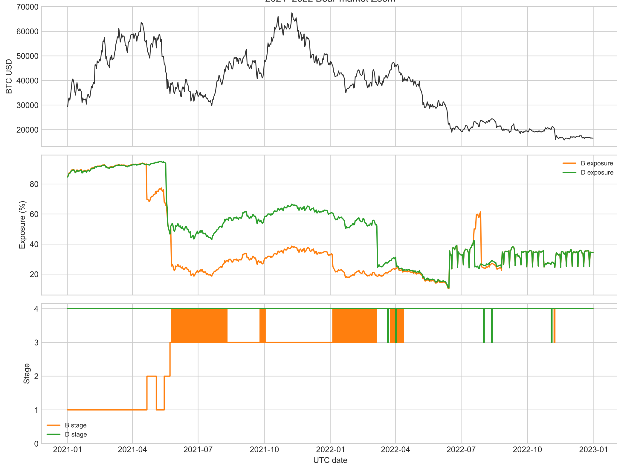
2021–2022 Bear-market Zoom
