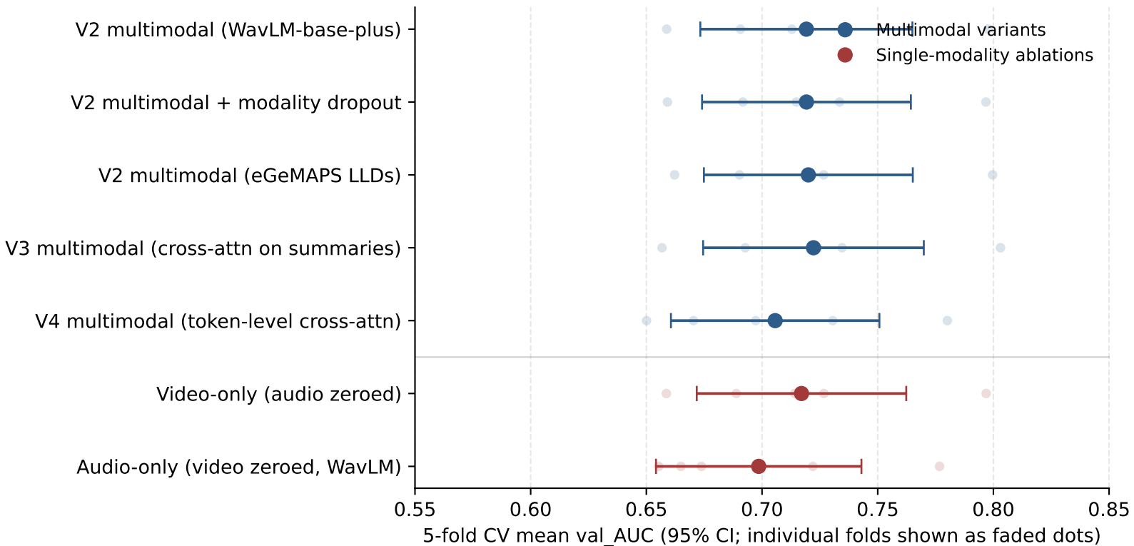
Multimodal synchrony classifier: CV mean val_AUC across conditions
