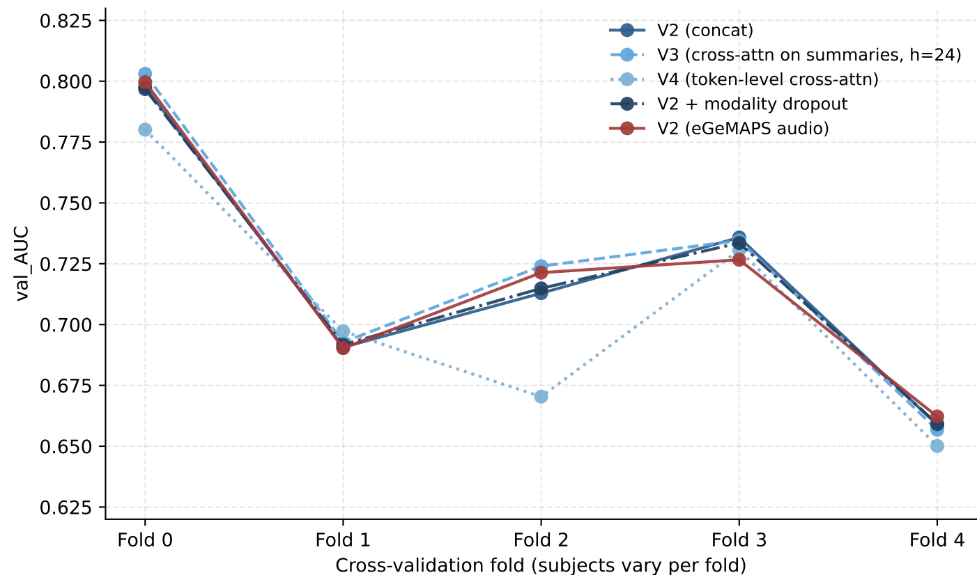
Per-fold val_AUC: fold rank is constant across architectures (architecture-to-architecture spread at any fold \ll fold-to-fold spread)
