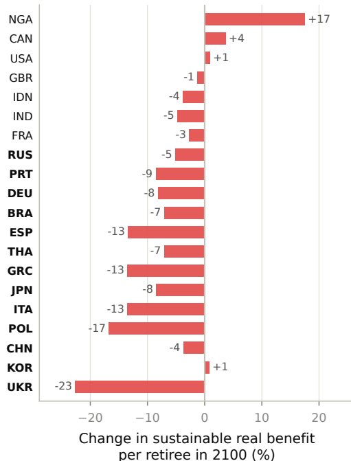
b What the elasticity decides: \varepsilon=1.00 vs fitted posterior
