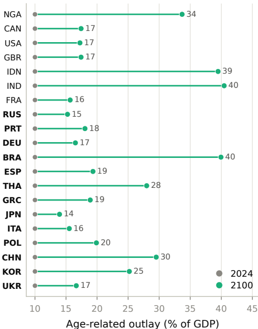
a Demographic pressure, 2024 → 2100: the same under either elasticity
