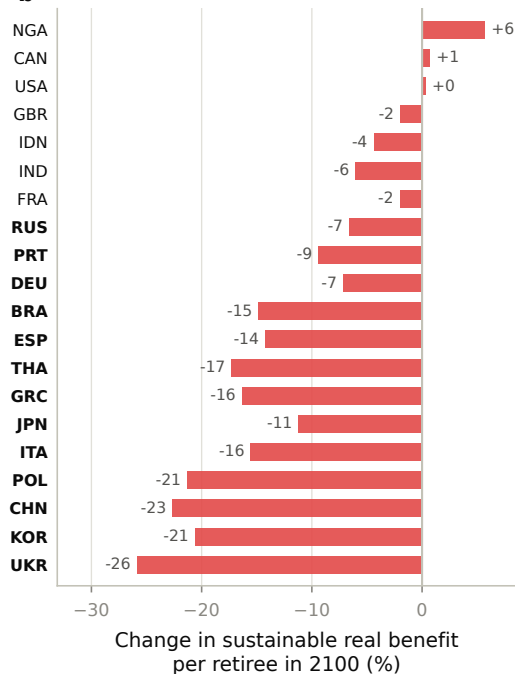
b What the elasticity decides: \varepsilon=1.22 world vs \varepsilon=0.92 world
