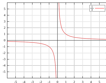
Fig. 1 Graph of the function y = 1/x , demonstrating the asymptotic behavior as x approaches zero and as x approaches infinity. The function never reaches x = 0 or y = 0 , but approaches them asymptotically. 1
