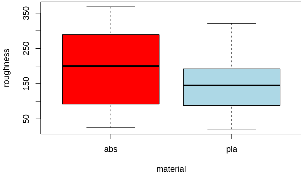
Boxplot roughness theo material
