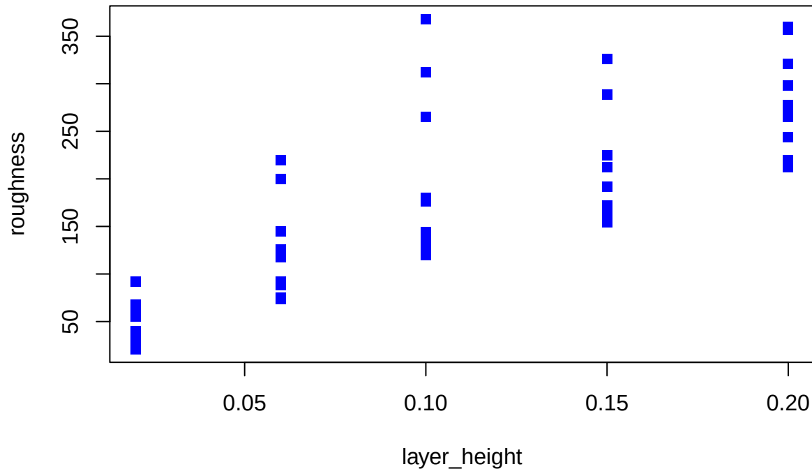
Scatter: layer_height vs roughness
