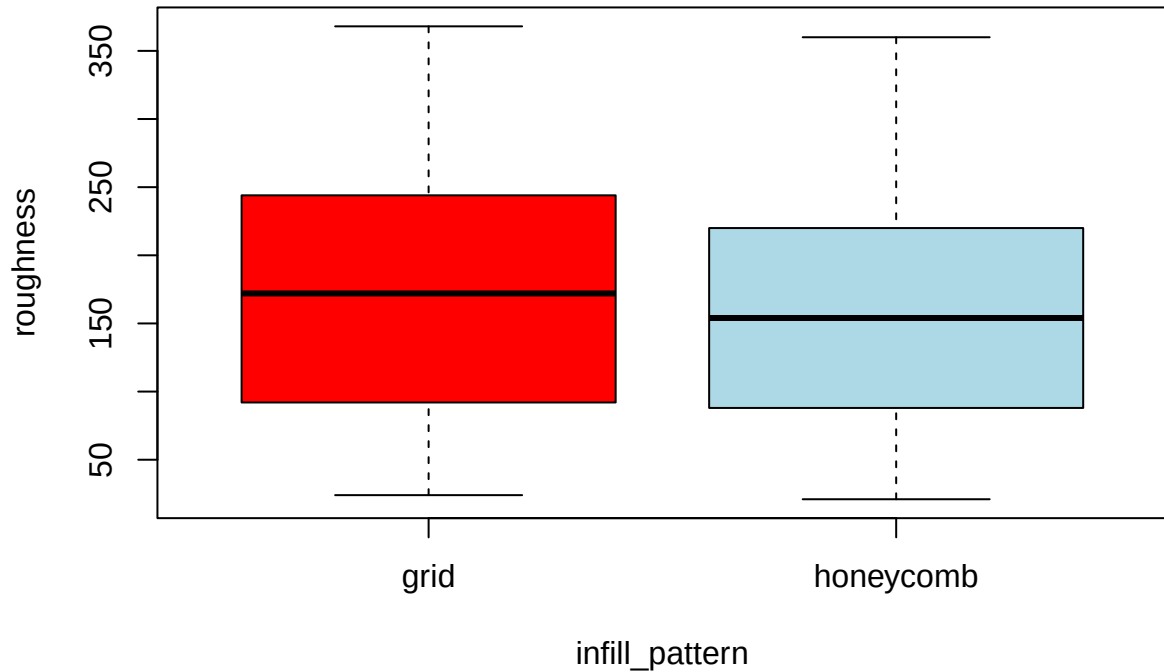
Boxplot roughness theo infill_pattern
