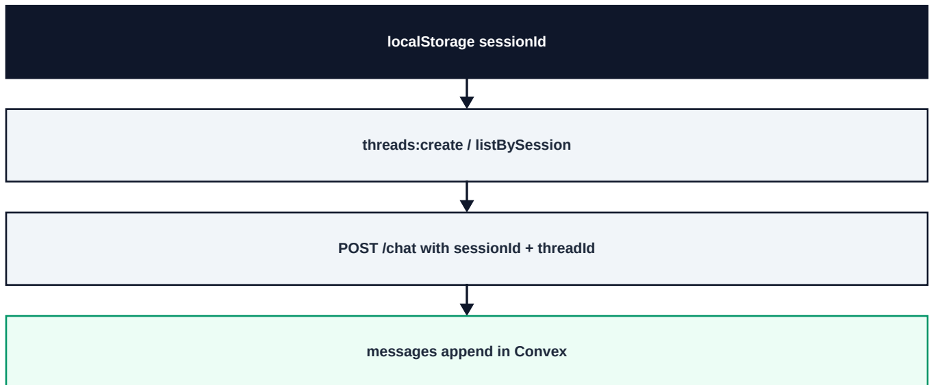
Figure 1. Auth surface for MVP.
