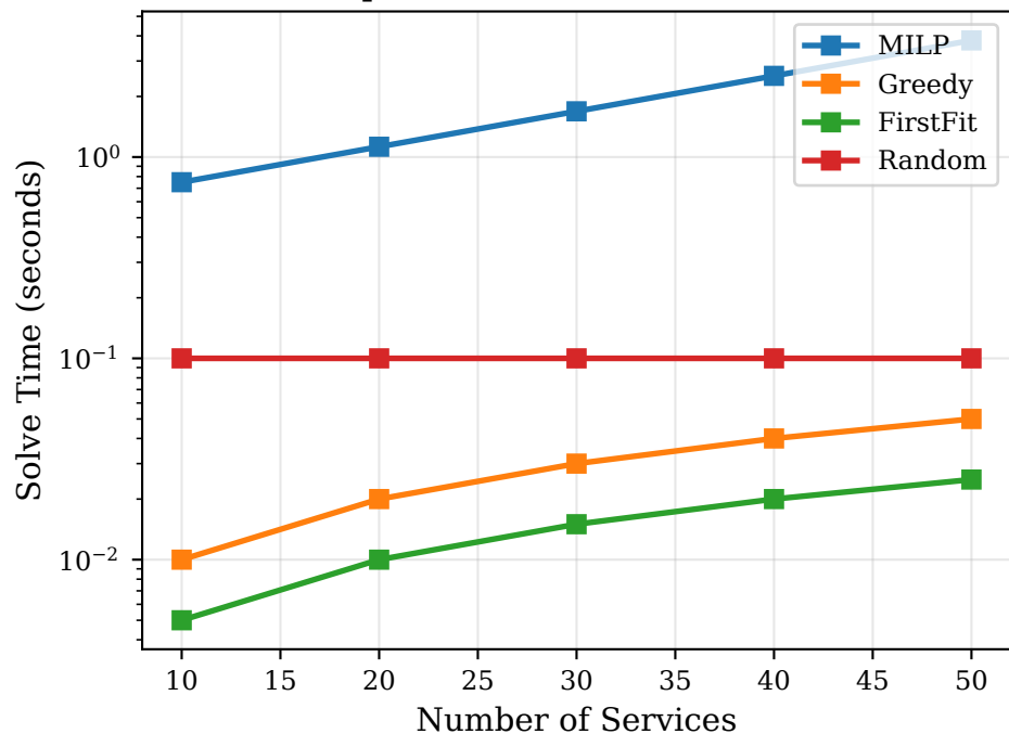
(b) Computational Time vs Problem Size
