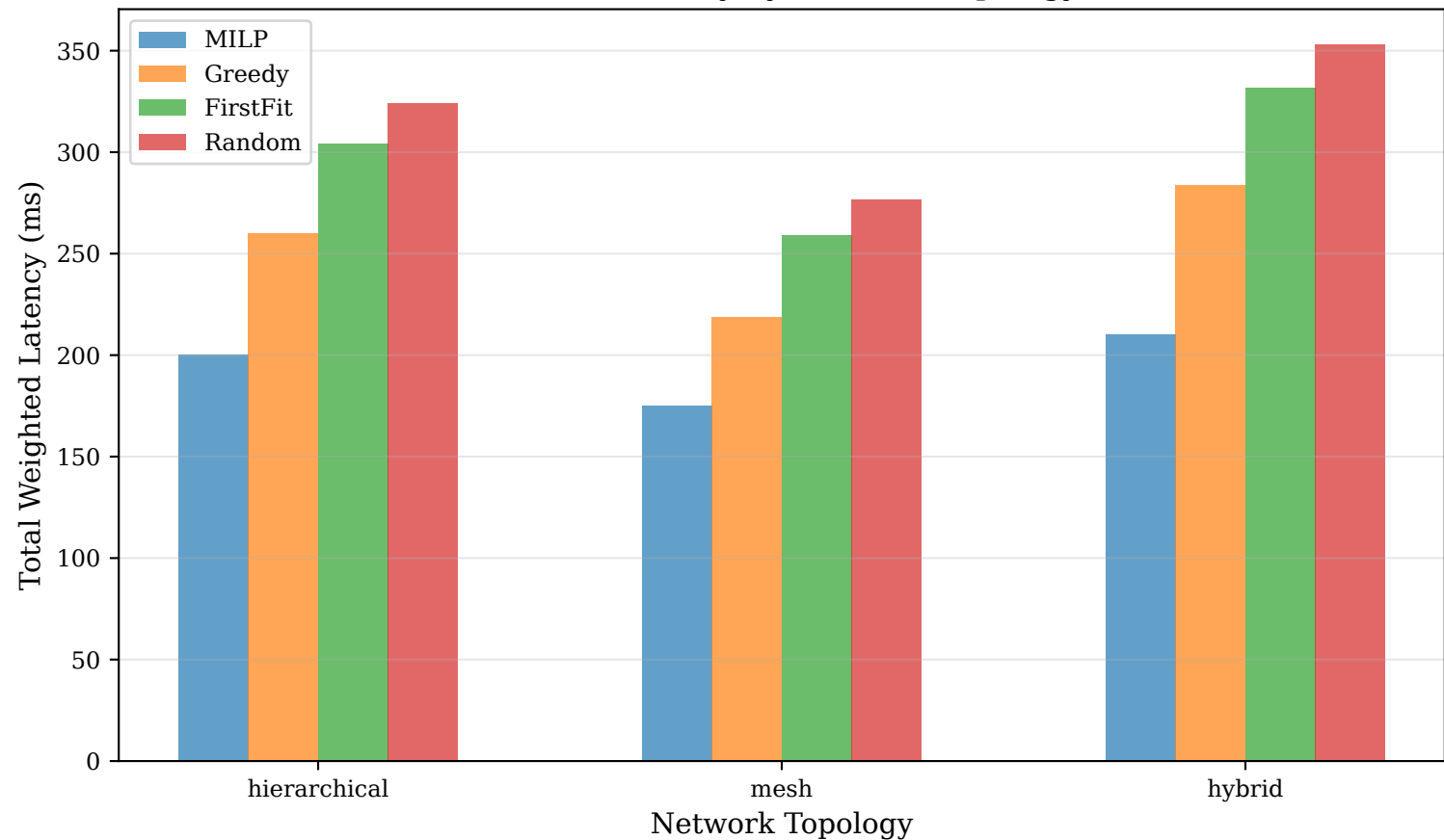
Solution Quality by Network Topology
