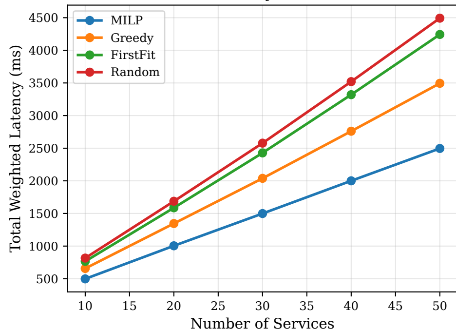
(a) Solution Quality vs Problem Size
