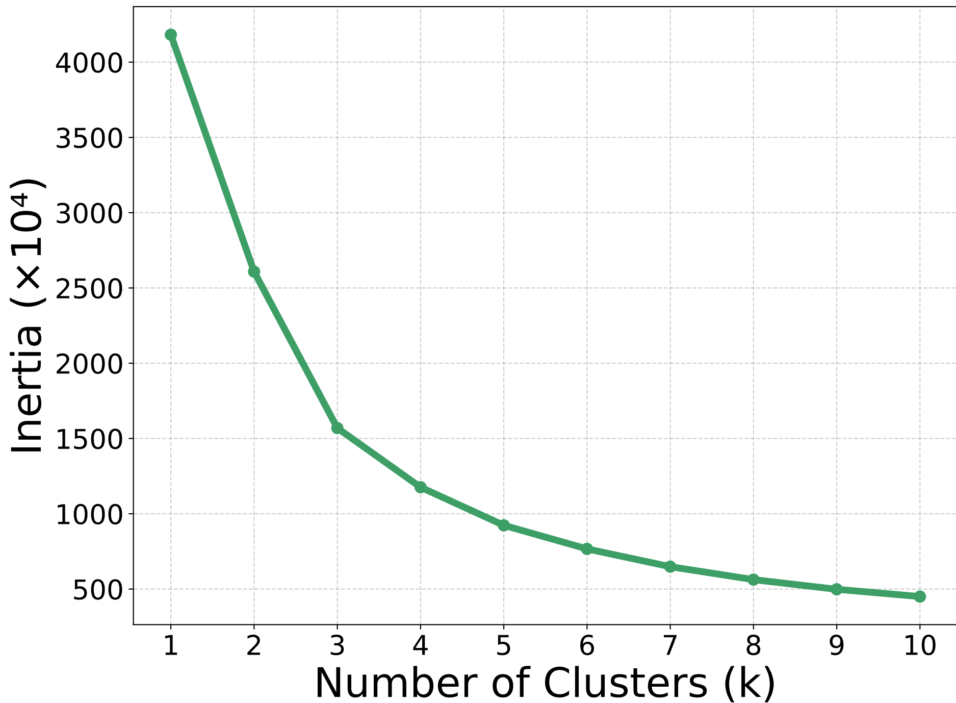
Elbow Method - t-SNE-reduced data
