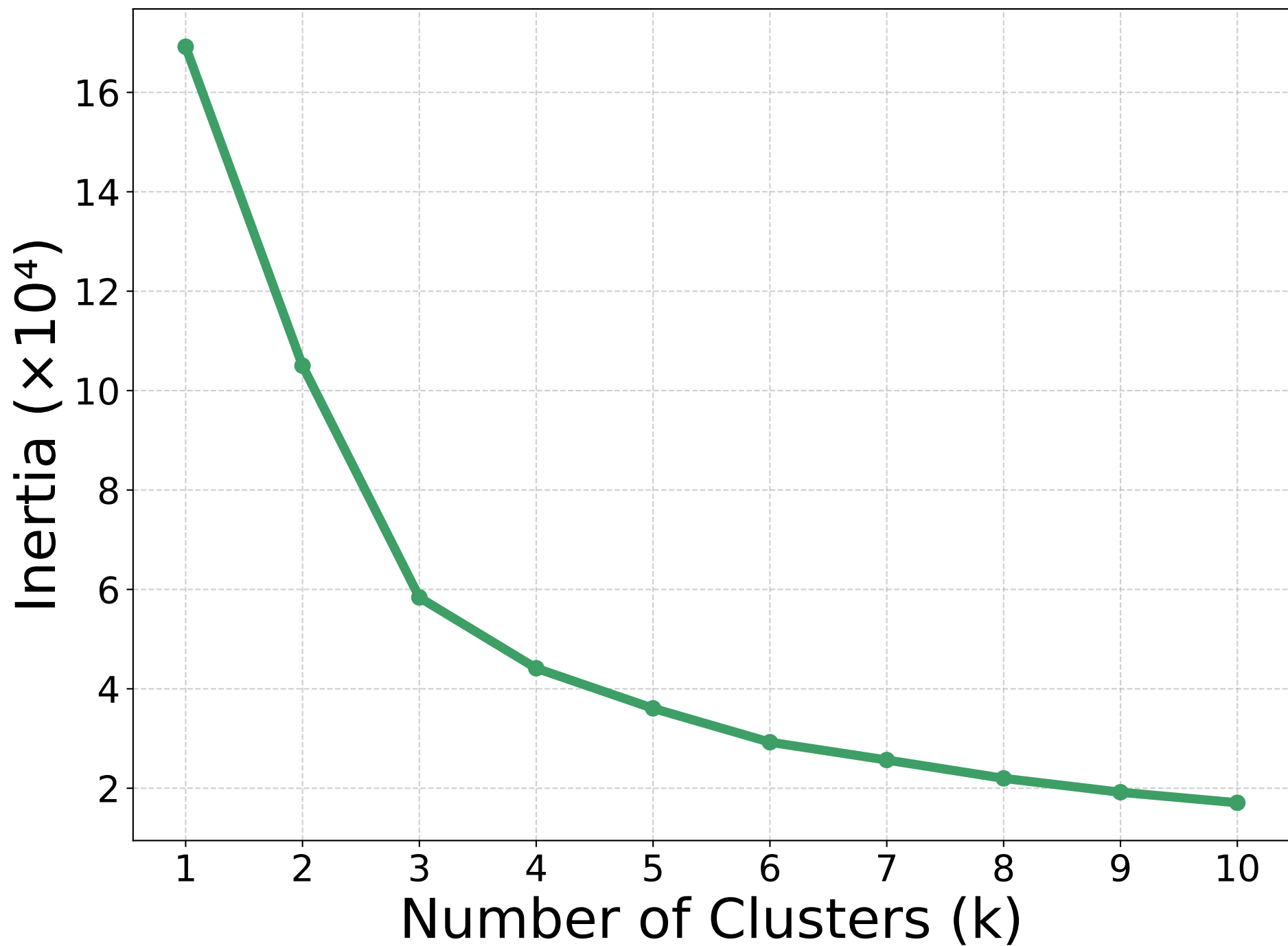
Elbow Method - UMAP-reduced data
