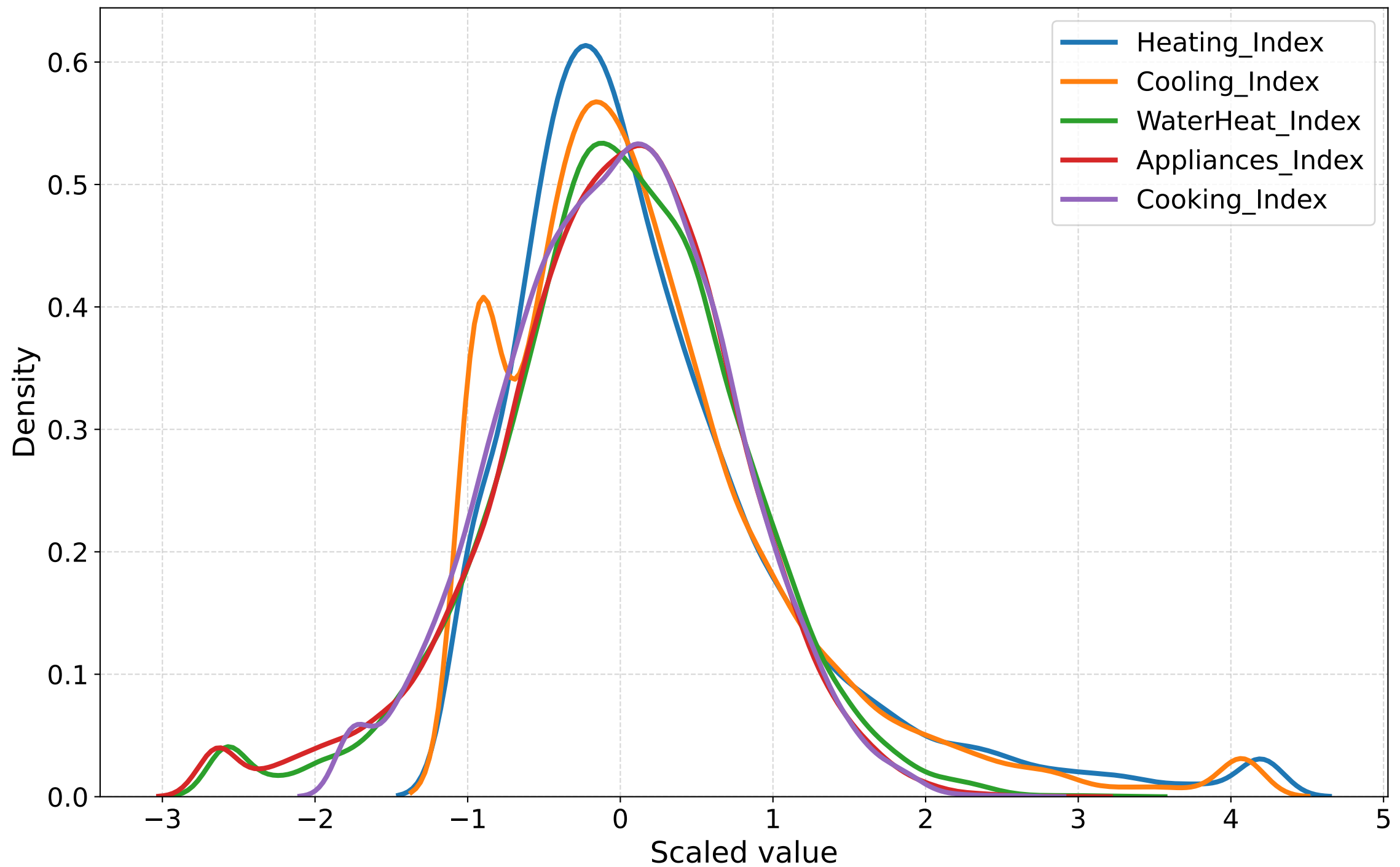
Kernel Density Estimation of Scaled Energy Variables
