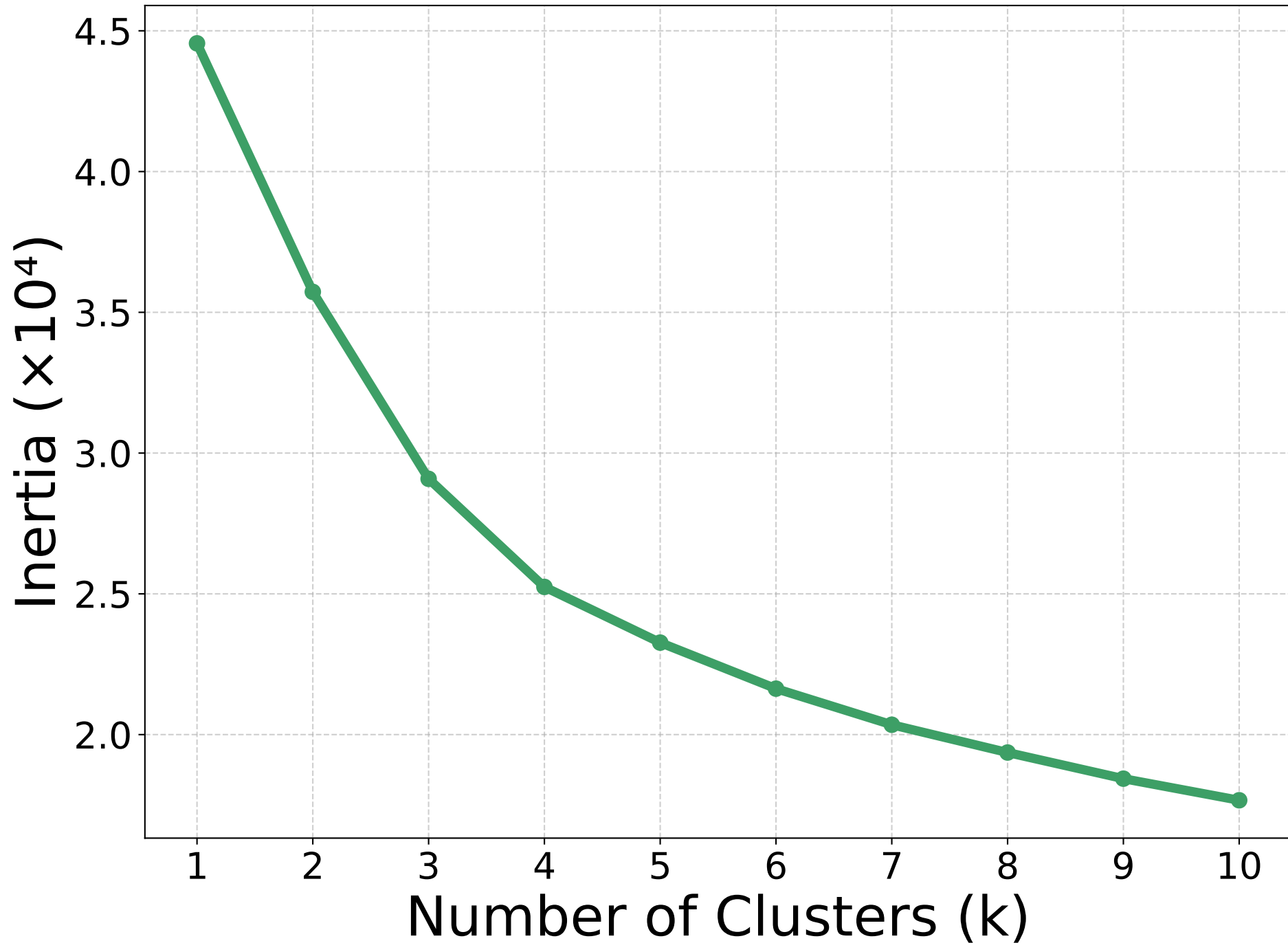
Elbow Method - original dataset
