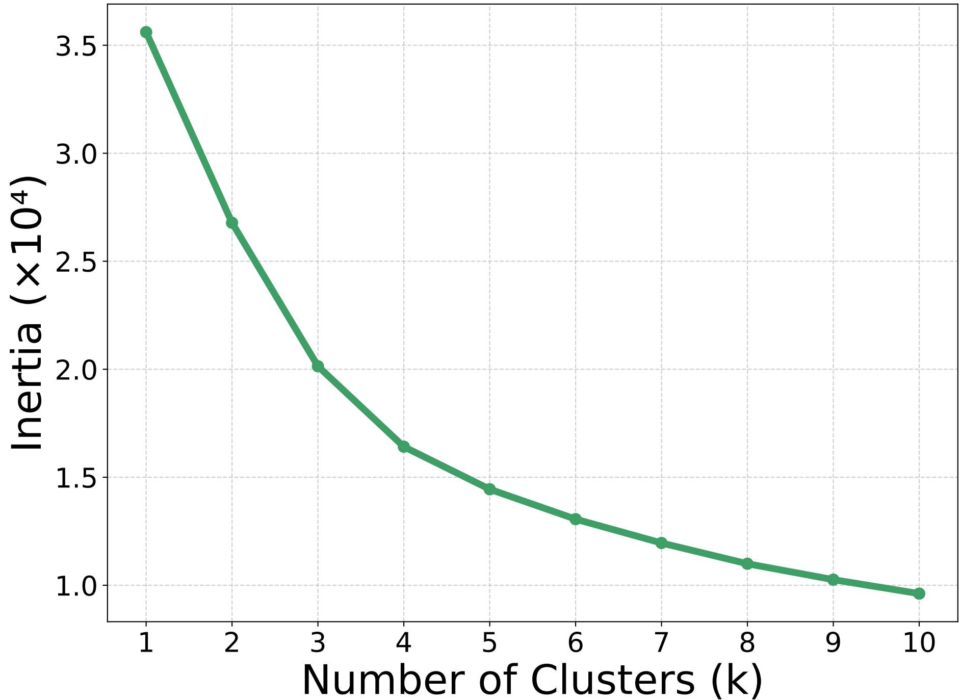
Elbow Method - PCA-reduced data
