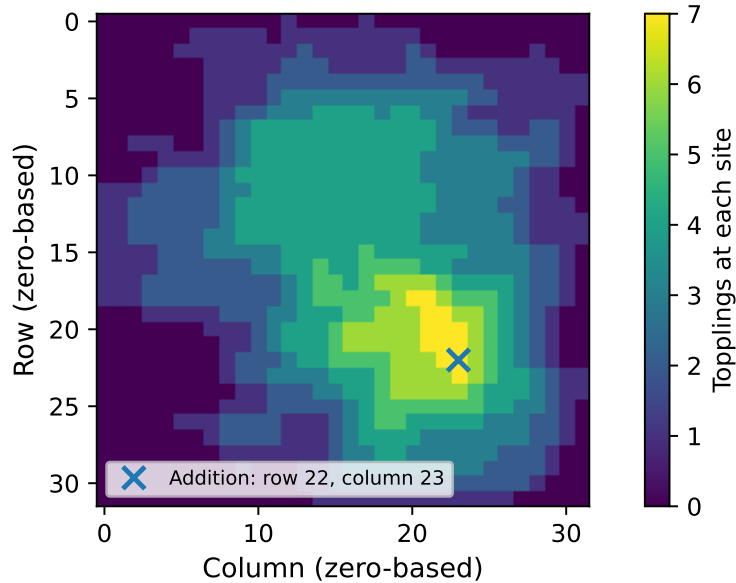
Figure 2: Site-level topplings for the largest recorded avalanche in BTW L = 32 , run 0. It occurs at post-burn-in addition 13,646 and has s = 2,145 , a = 768 , d = 29 and r = 27.0185 . The cross marks zero-based row 22, column 23; a site topples at most seven times. This is a selected large event from one run.
