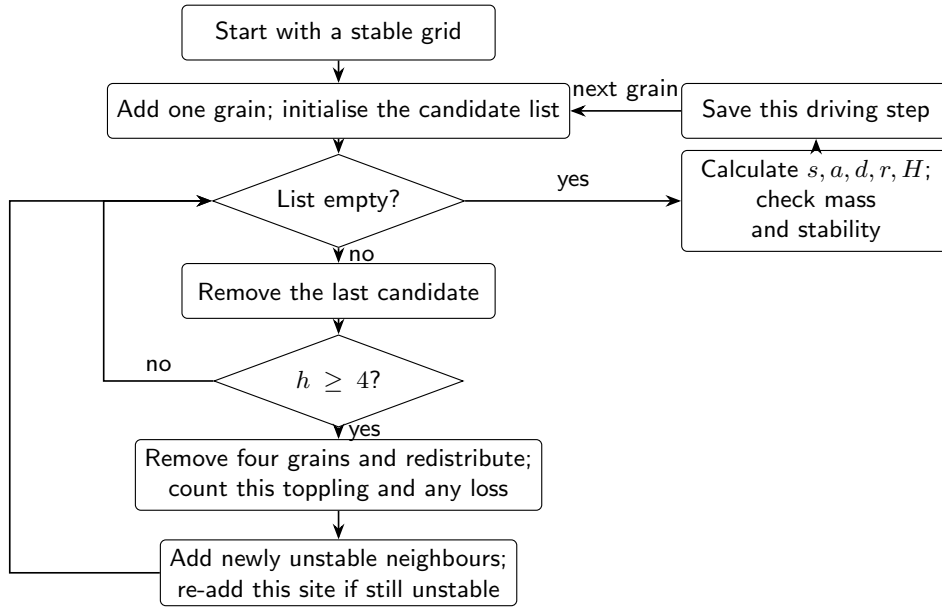
Figure 1: Candidate-list algorithm for one grain addition and complete relaxation. The same loop handles both rules; only the choice of outgoing directions changes. A new driving step starts after the candidate list is empty and the checks have passed.
