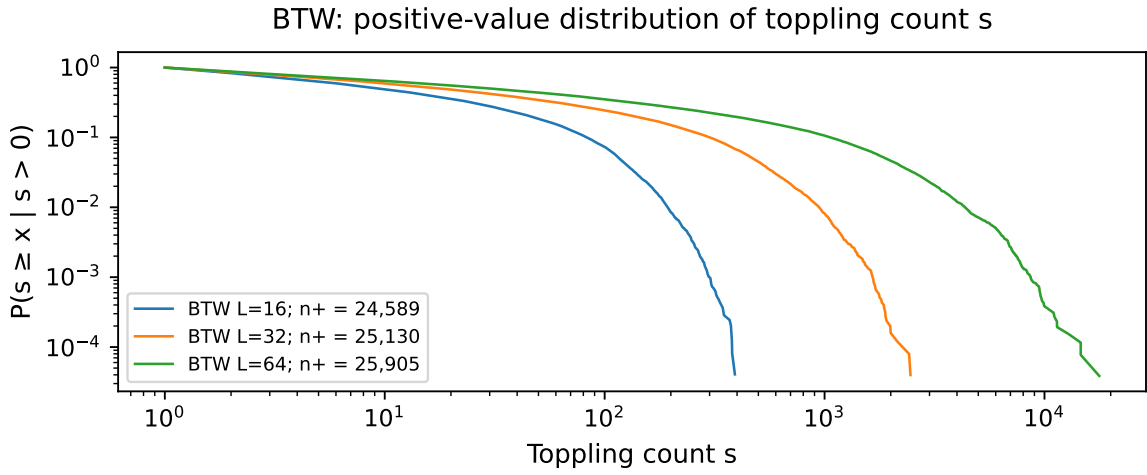
Figure 6: Positive-value CCDF of the number of topplings. Each curve pools three runs, each with 20,000 recorded additions. The legend gives the number of nonzero observations. The larger- L curves extend to substantially greater toppling counts.
