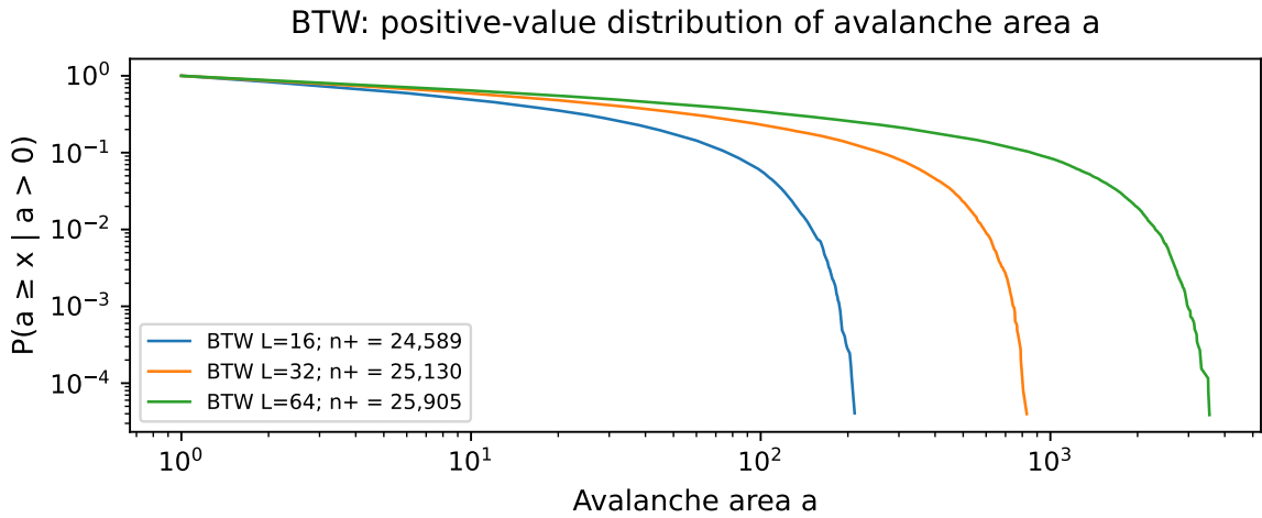
Figure 7: Positive-value CCDF of avalanche area for the same runs. The positive sample counts equal those for s , because an avalanche has at least one toppled site. Area is bounded by L^2 ; repeated topplings do not add new sites.
