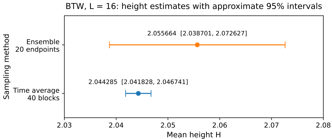
Figure 5: Time and ensemble estimates for mean height at L = 16 . Horizontal intervals use Student- t multipliers. The time interval treats 40 block means as approximately independent; the ensemble interval uses 20 independent endpoints. Numerical values are also given in Table 3.
