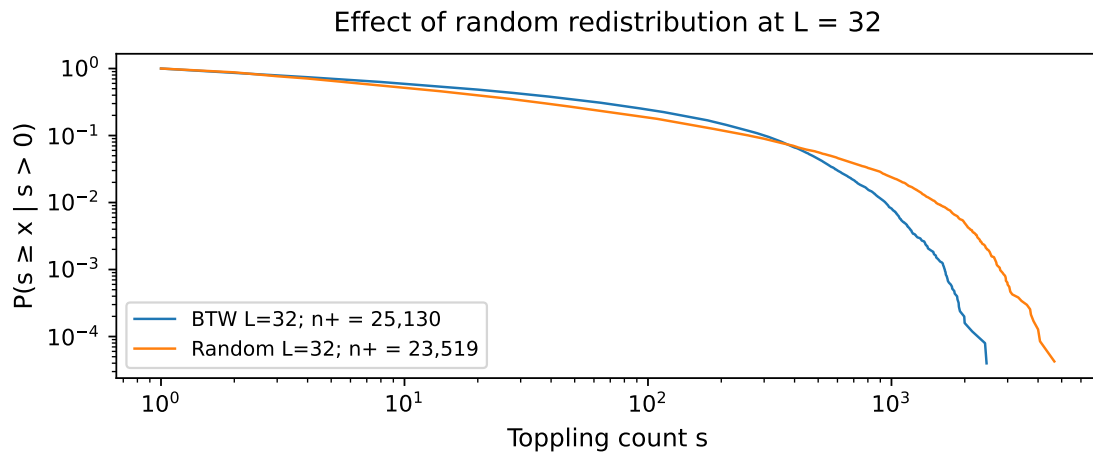
Figure 12: Positive toppling-count distributions at L = 32 , pooling the three runs per rule. The curves cross, so their ordering depends on the threshold examined. Table 8 reports specific run-level means and quantiles, with their conditioning stated explicitly.
