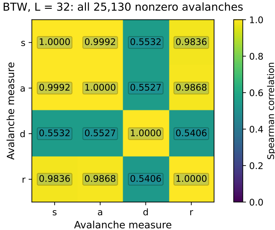
Figure 10: Spearman correlations among all 25,130 nonzero BTW avalanches at L = 32 , pooled across three runs. Zero loss and zero radius are retained. Displayed values use four decimal places and match the BTW column of Table 6.
