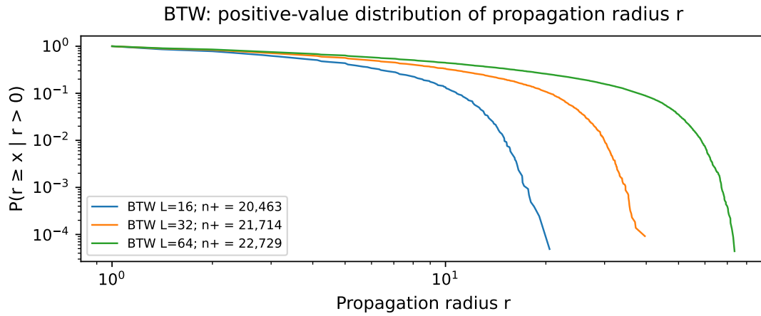
Figure 9: Propagation radius conditional on r > 0 . Distances are Euclidean with unit lattice spacing. The bound is r \leq \sqrt{2}(L-1) . The outward shift with L reflects the larger available spatial extent.
