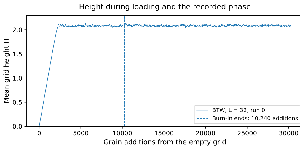
Figure 3: Mean height in BTW L = 32 , run 0, from the empty grid through the recorded phase. The vertical line marks the end of 10,240 burn-in additions. Every 25th step is displayed; all steps are used in the calculations. This single trajectory is distinct from the three-run summaries below.
