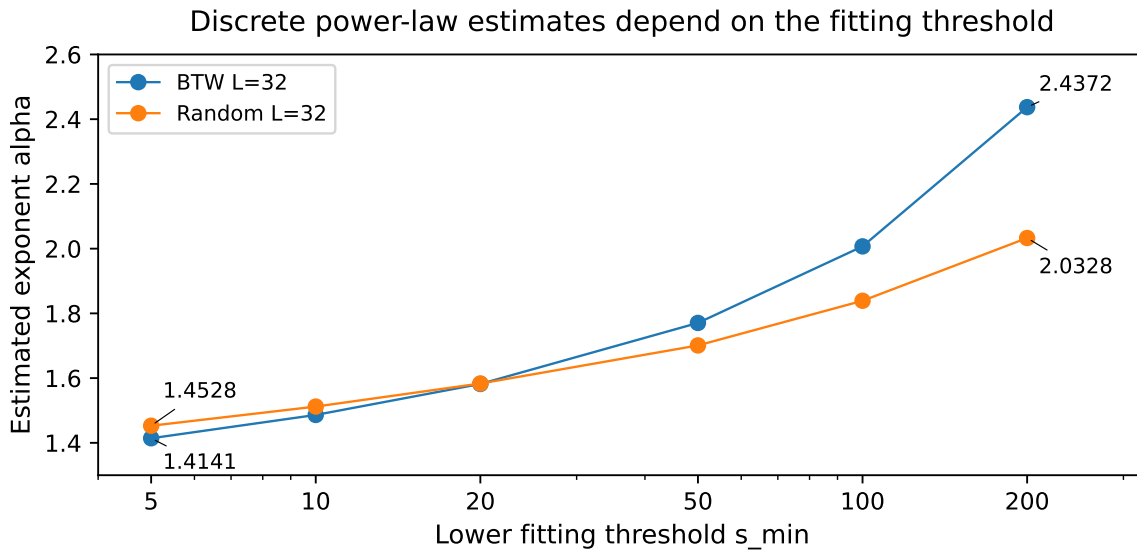
Figure 11: Exploratory discrete maximum-likelihood estimates for the two L = 32 settings. Points use the same six thresholds. The labels identify the endpoint estimates; the line segments simply join the estimates. No confidence intervals are claimed.
