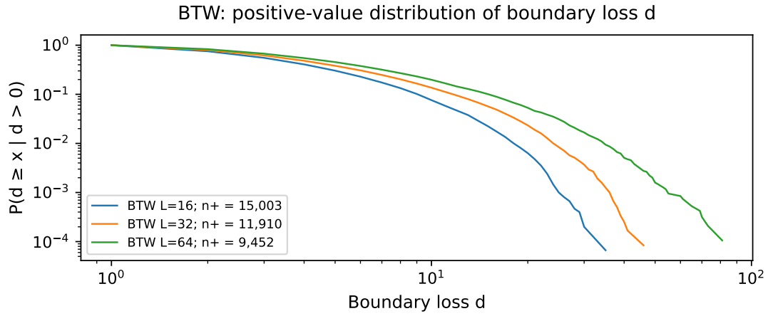
Figure 8: Boundary loss conditional on d > 0 . Larger grids have fewer loss-producing additions in these records (Table 5), although positive loss events can be larger. Mean loss over all additions stays close to one.
