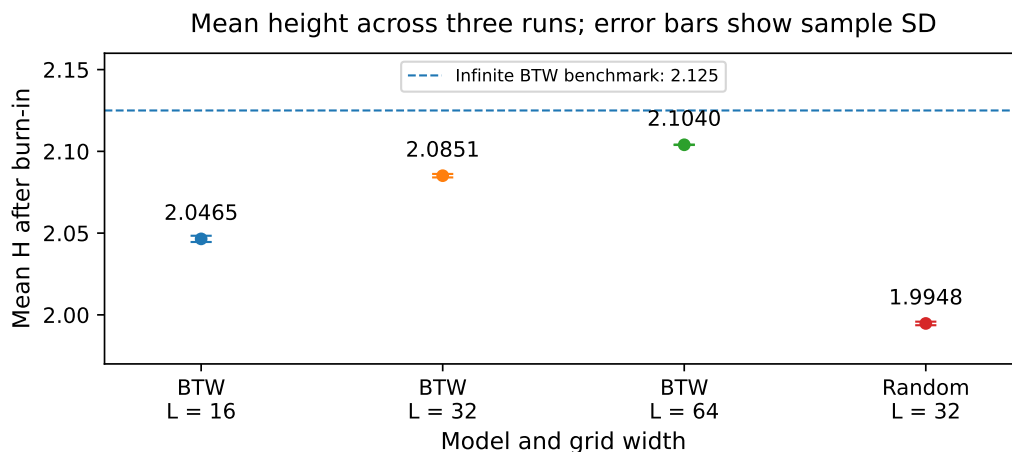
Figure 4: Mean post-burn-in height across three runs per setting. The labels are rounded to four decimal places; error bars show run-to-run sample SD. The random-rule value is included for the later comparison. The dashed benchmark applies to infinite-lattice BTW.
