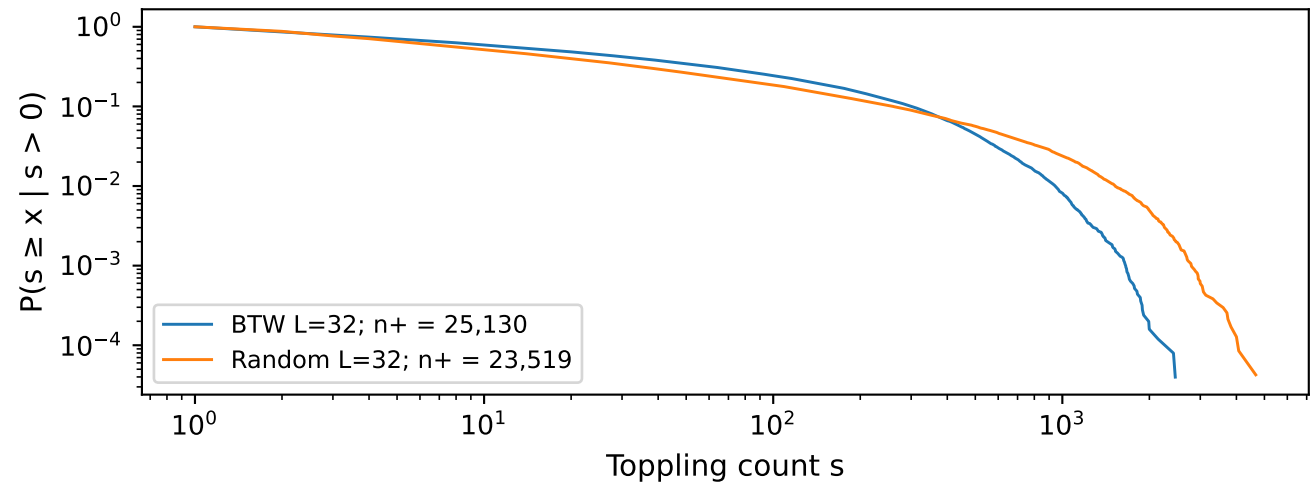
Effect of random redistribution at L = 32
