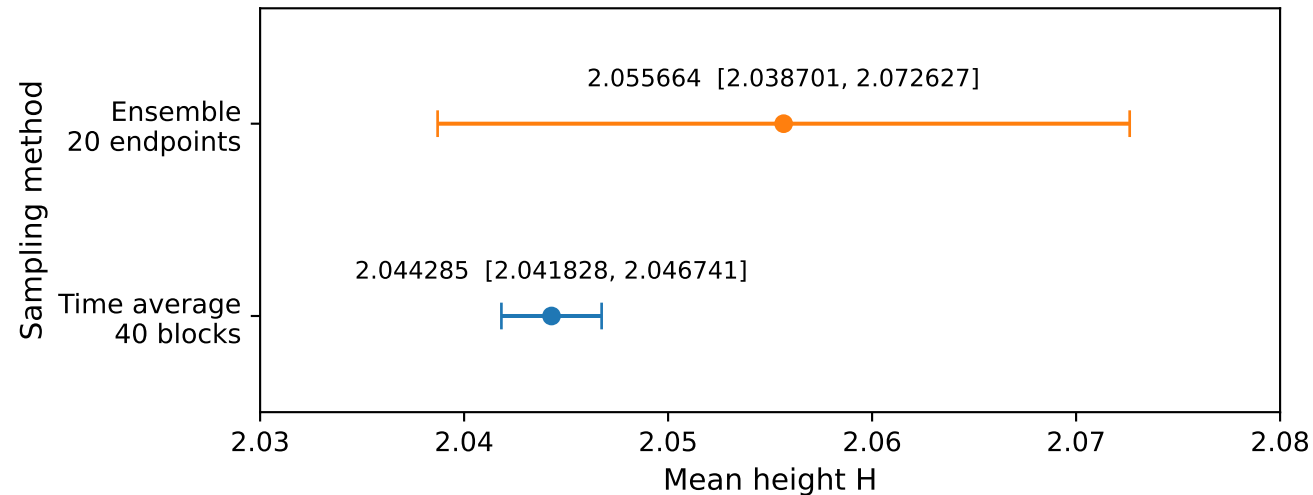
BTW, L = 16: height estimates with approximate 95% intervals
