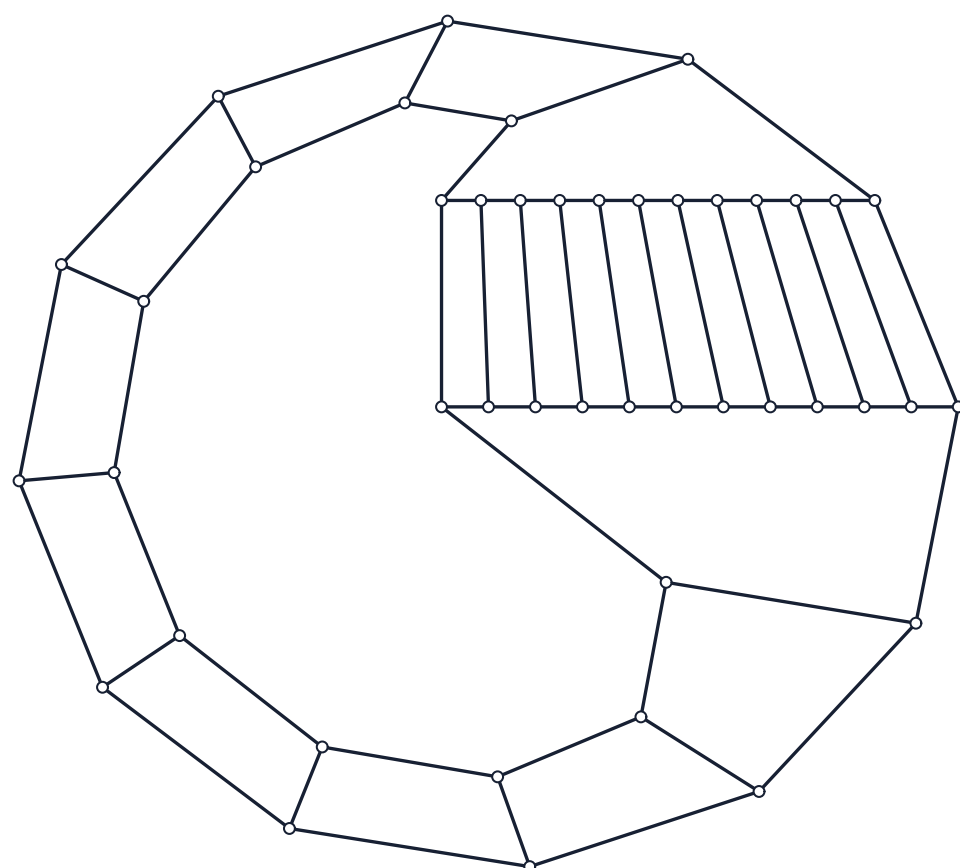
D(7,5) n=28 hsep=31 [certified]
