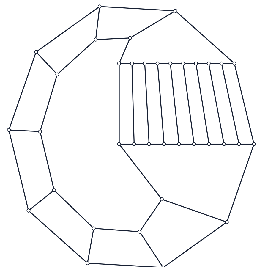
D(5,3) n=20 hsep=17 [certified]
