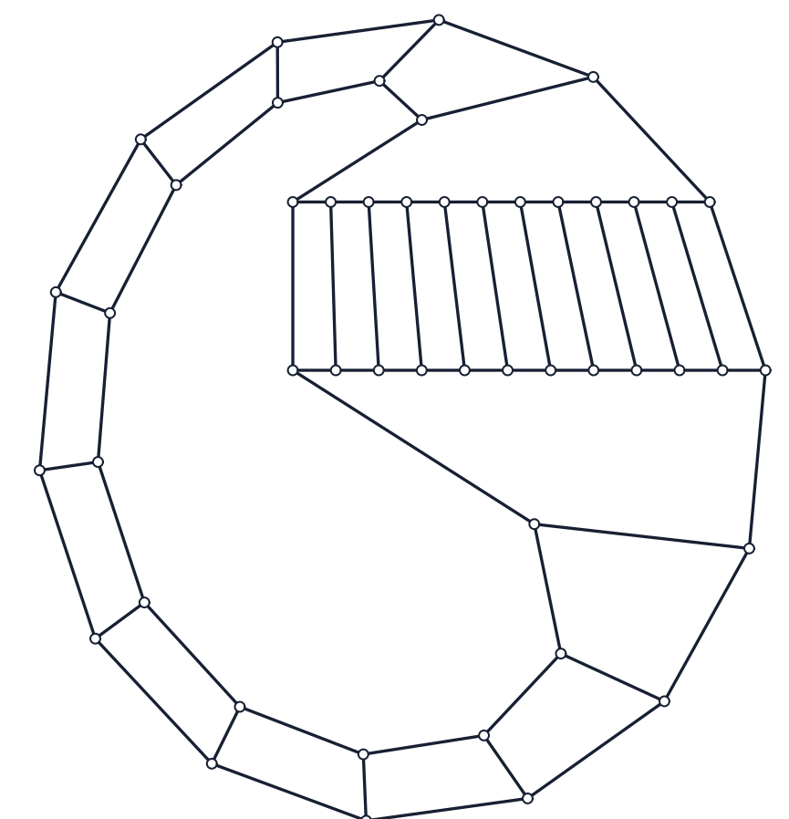
D(7,7) n=32 hsep=40 [certified]
