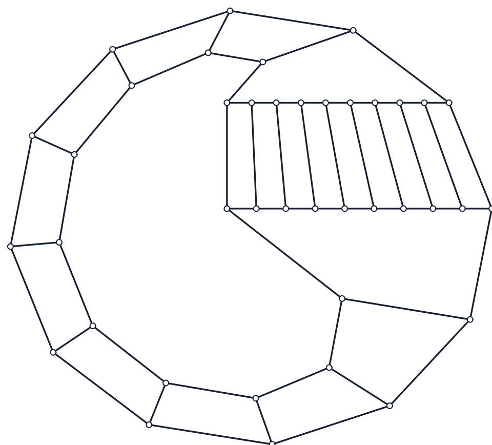
D(5,5) n=24 hsep=24 [certified]
