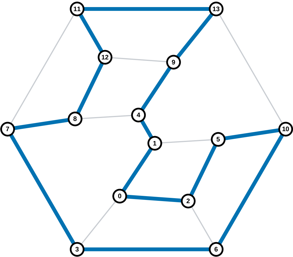
Hamiltonian cycle 2/12
