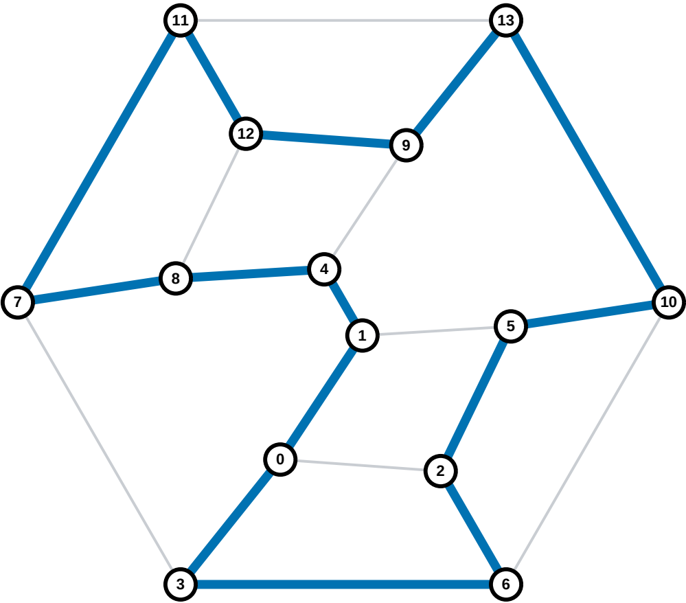
Hamiltonian cycle 5/12
