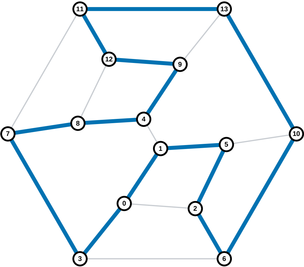
Hamiltonian cycle 7/12
