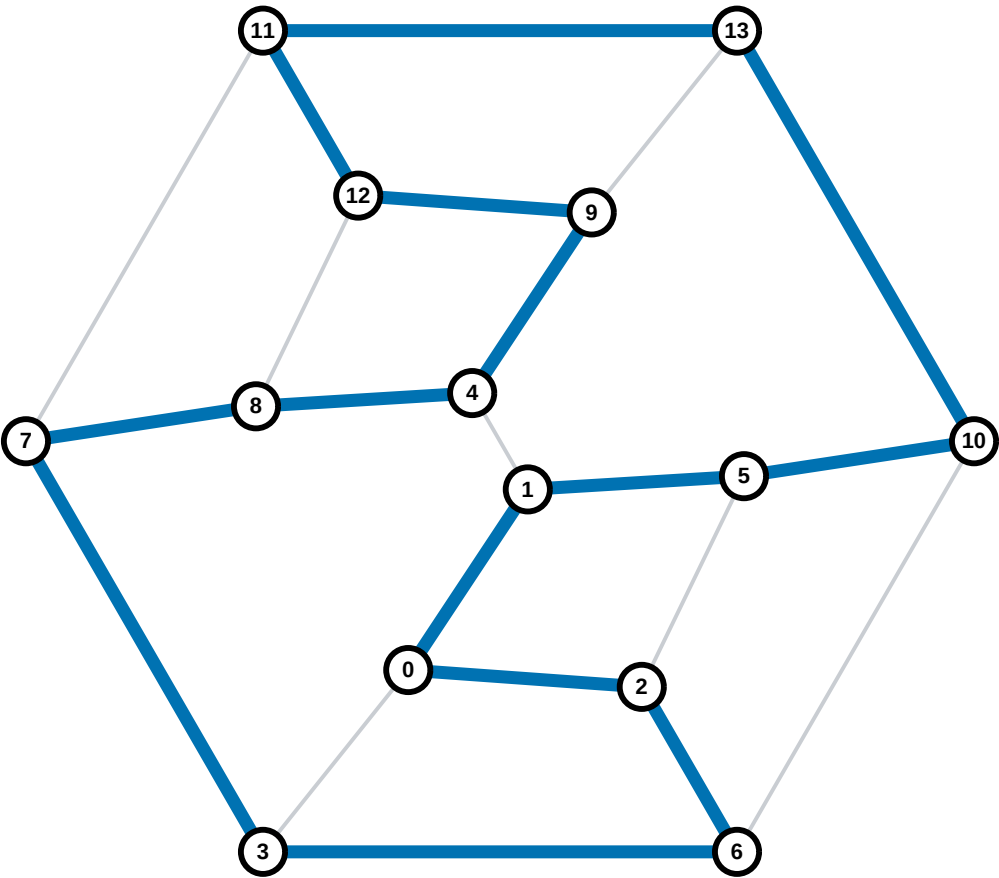
Hamiltonian cycle 3/12
