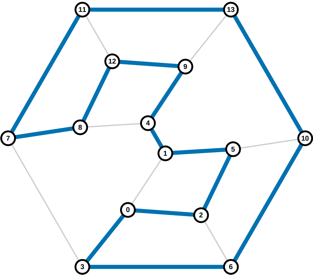
Hamiltonian cycle 10/12
