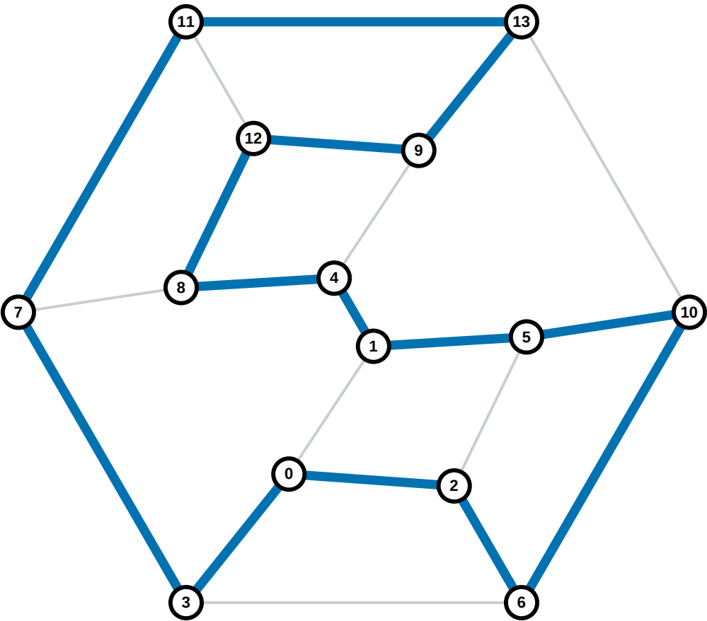
Hamiltonian cycle 11/12
