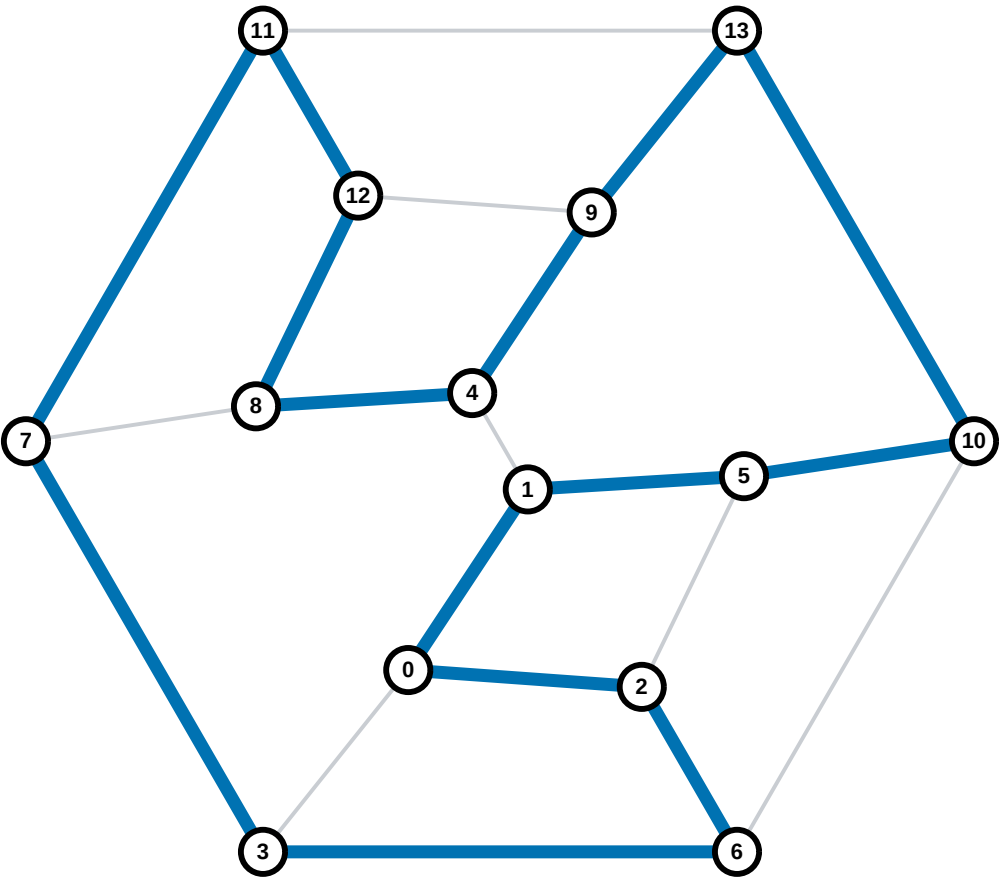
Hamiltonian cycle 4/12
