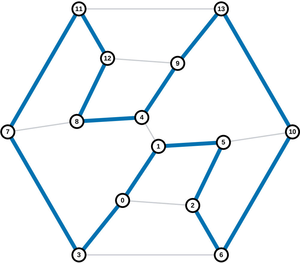
Hamiltonian cycle 8/12
