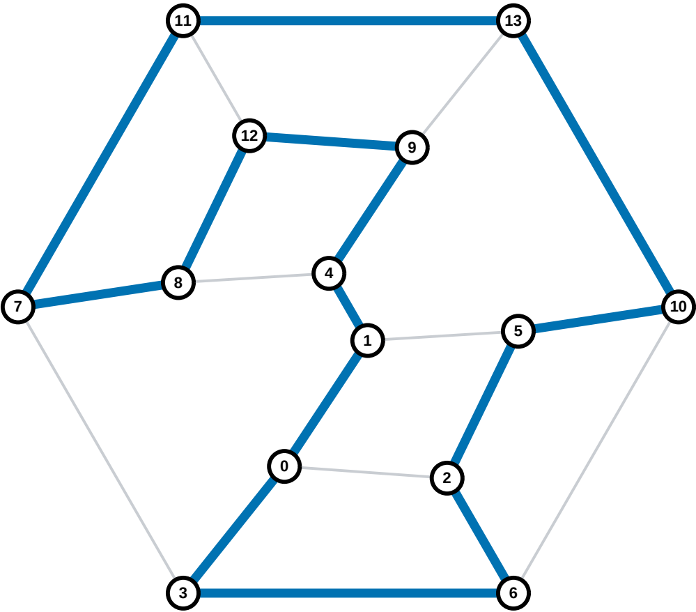
Hamiltonian cycle 6/12
