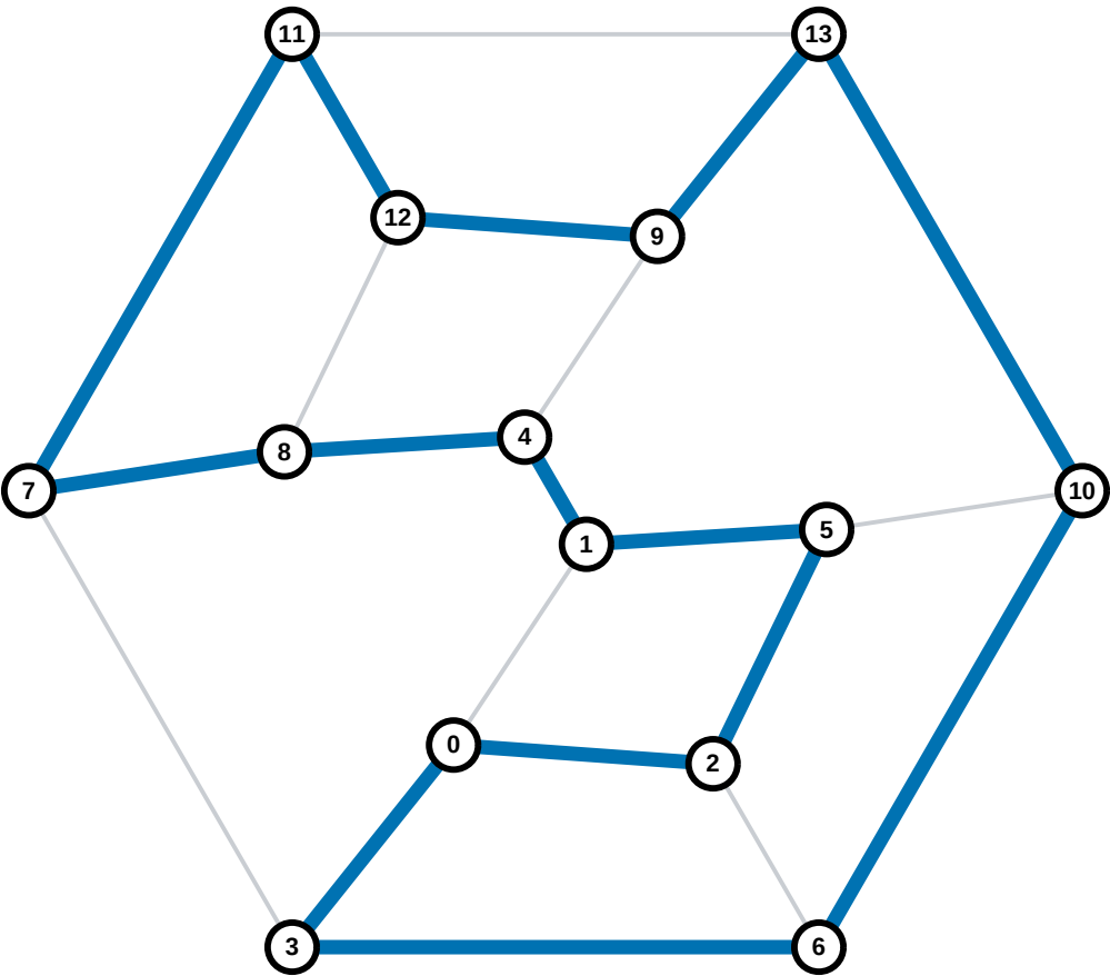
Hamiltonian cycle 9/12
