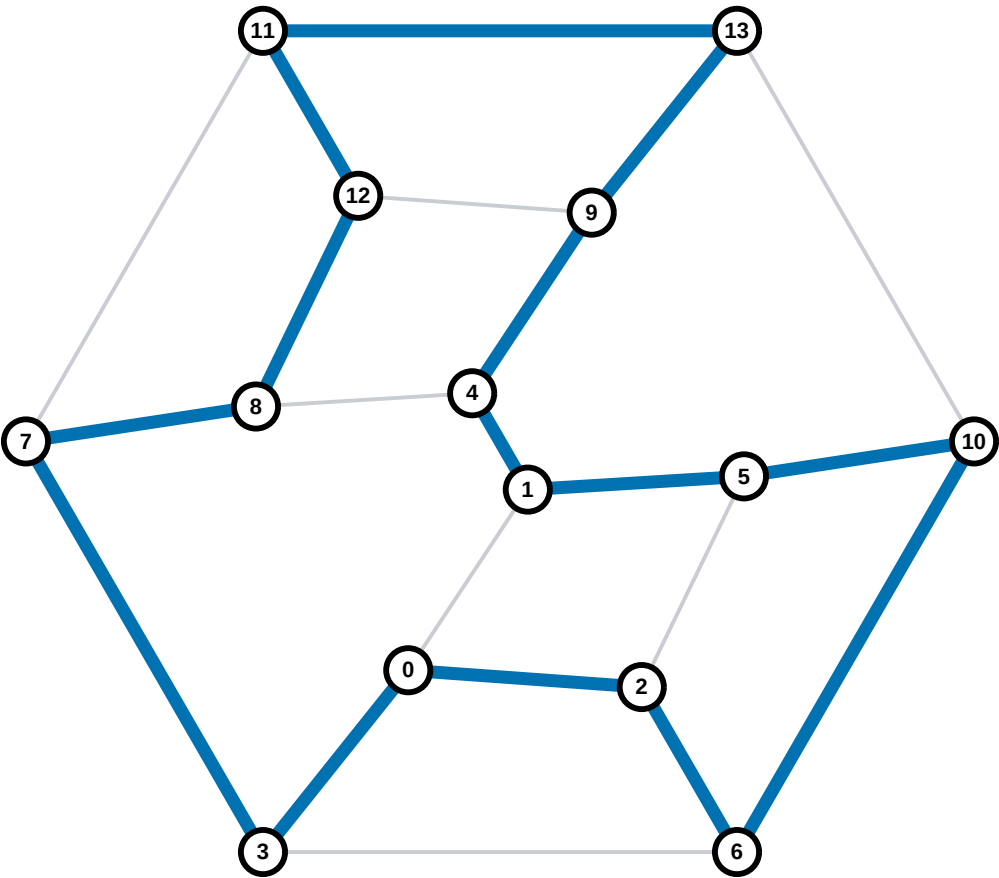
Hamiltonian cycle 12/12
