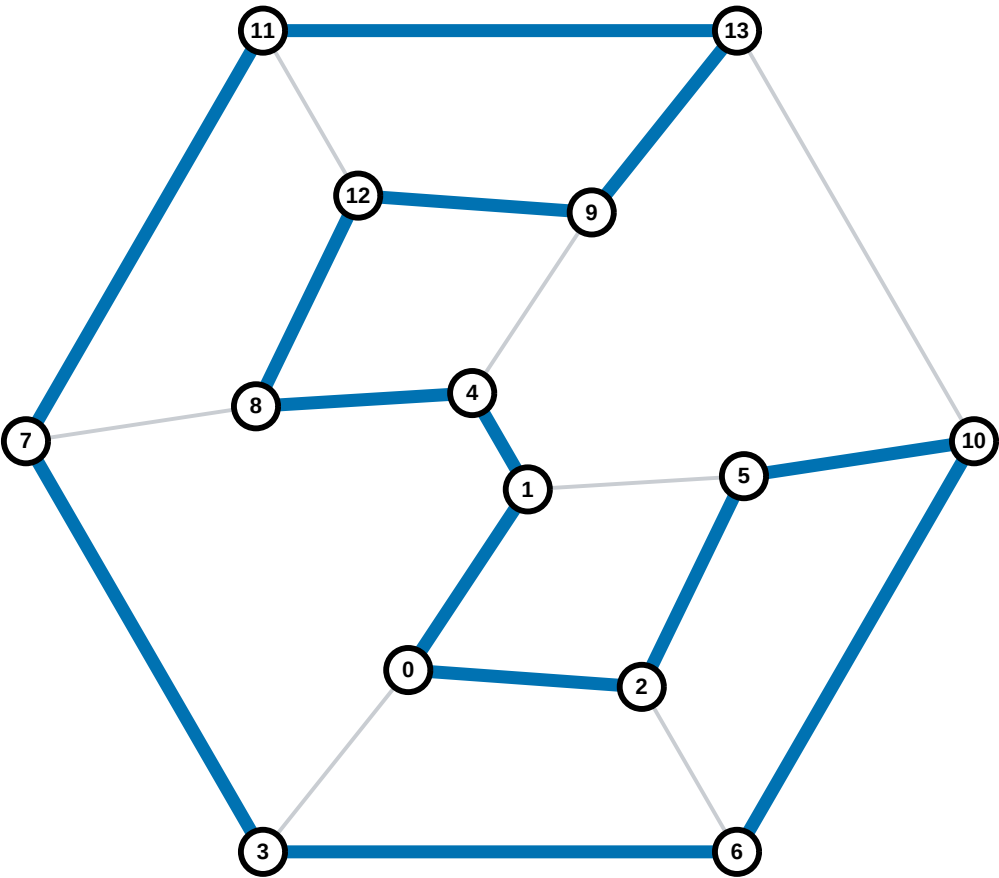
Hamiltonian cycle 1/12
