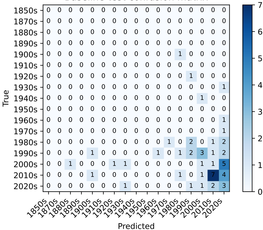
Baseline test confusion matrix
