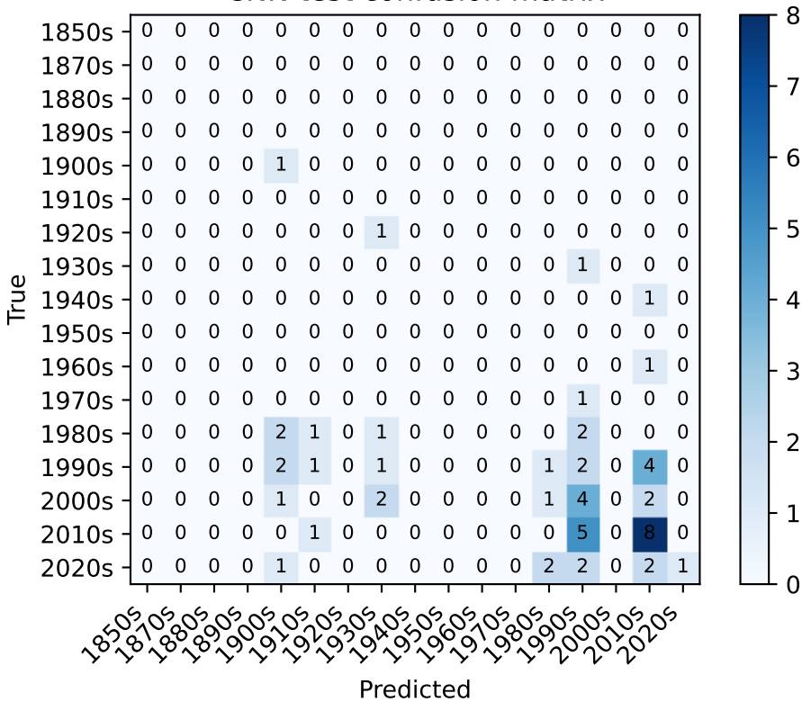
CNN test confusion matrix
