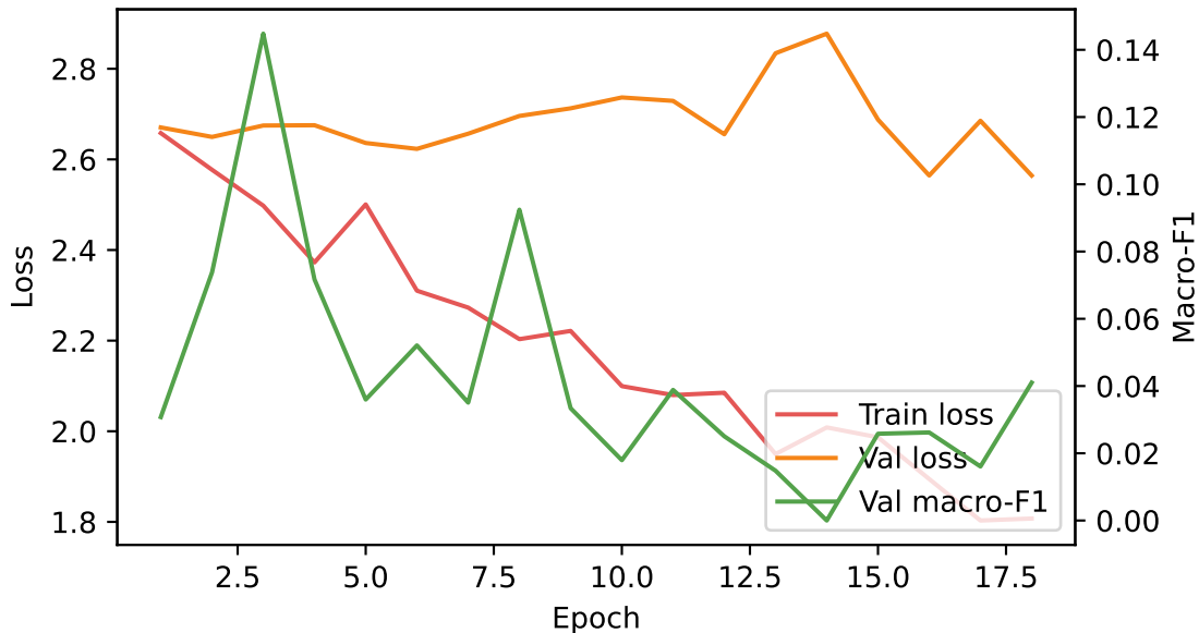
CNN training curve
