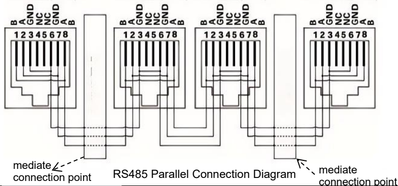
RJ45 Interface (X2-B) RJ45 Interface (X2-A) RJ45 Interface (X2-B) RJ45 Interface (X2-A)
