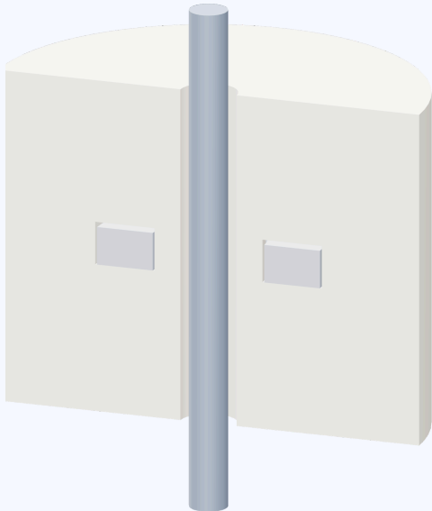
An explanatory 3.175 mm rod through the actual 4.8 mm float bore. This picture shows the guide interface, not measured liquid performance.
