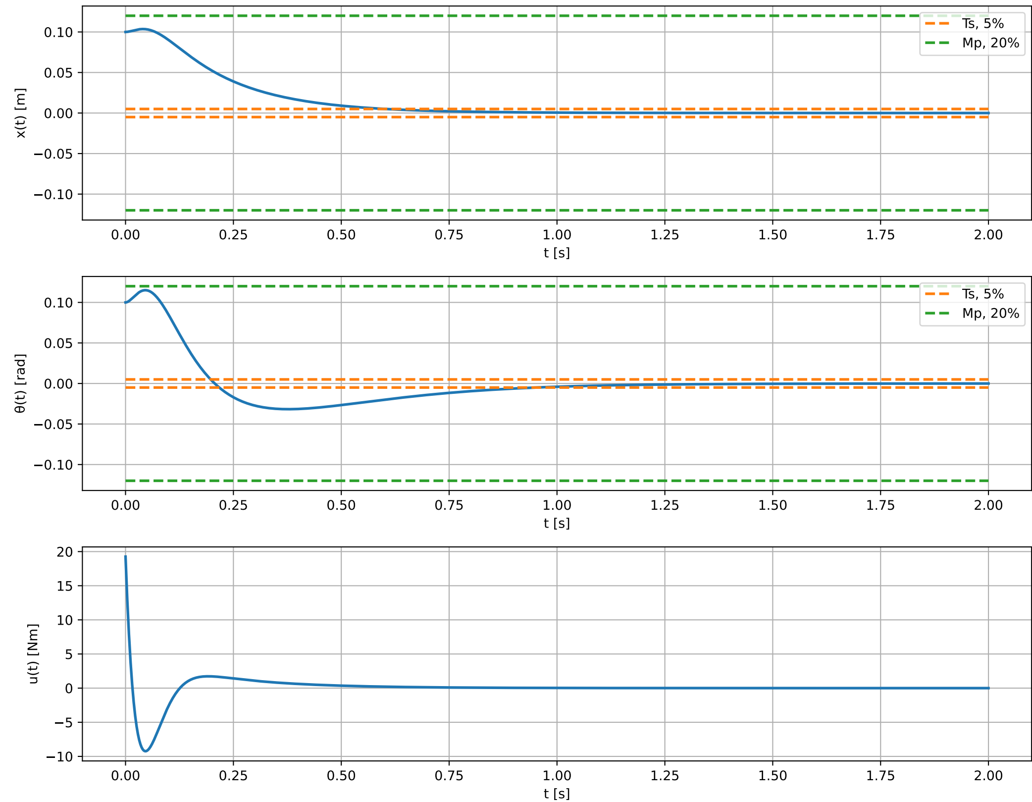
x(t) , \theta(t) , u(t) for cartpole under lqr control
