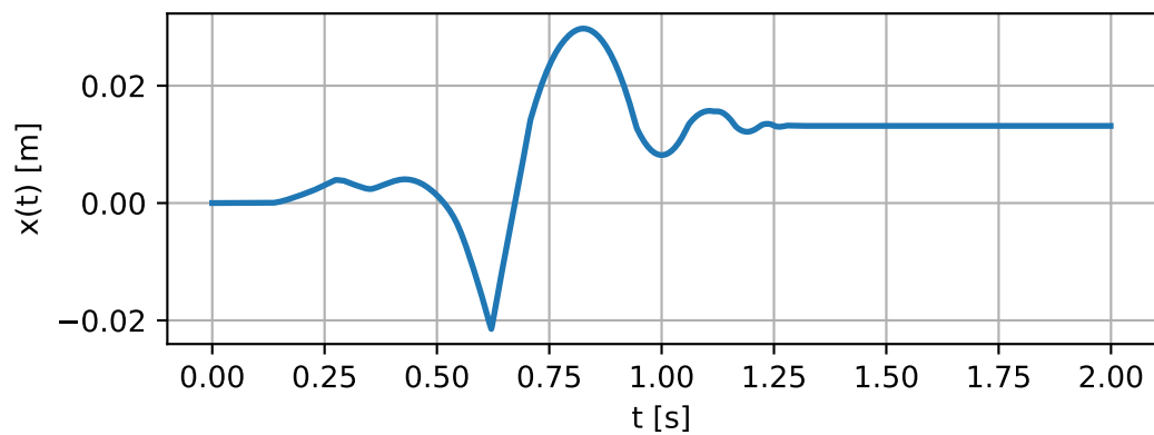
x(t) , \theta(t) , \tau(t) for balancing biped under mpc control
