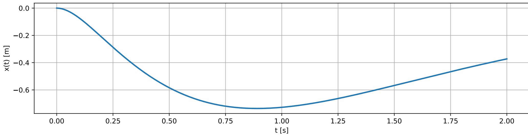
x(t) , \theta(t) , u(t) for cartpole under lqr control
