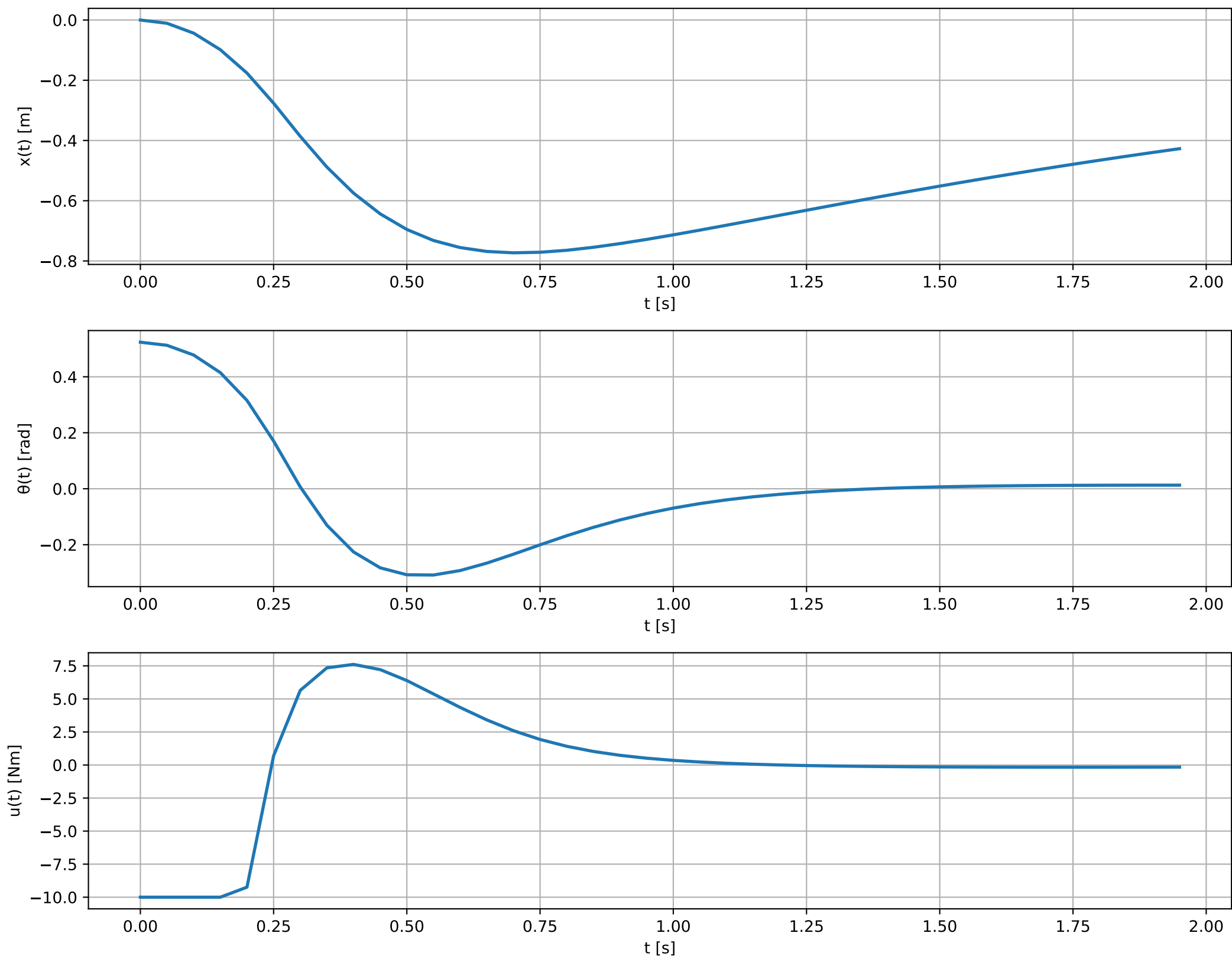
x(t) , \theta(t) , u(t) for cartpole under mpc
