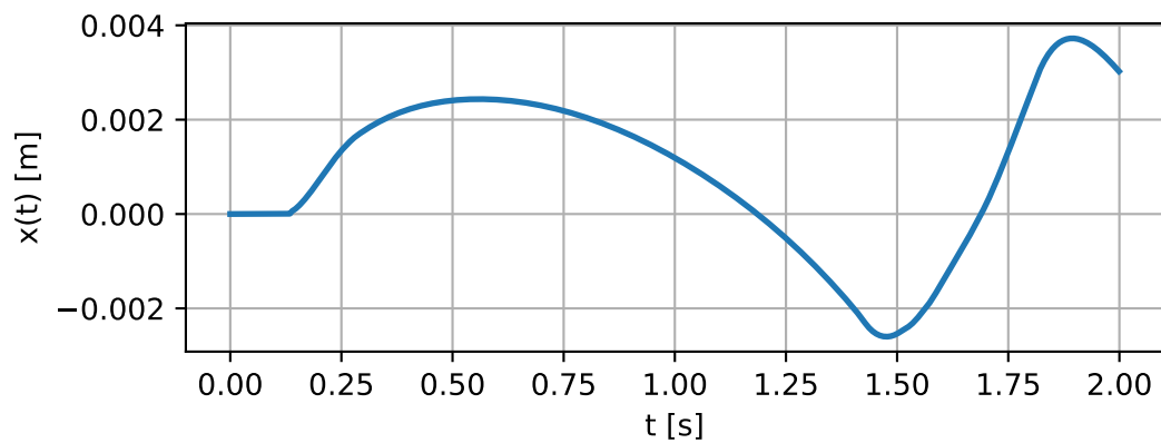
x(t) , \theta(t) , \tau(t) for balancing biped under qp control
