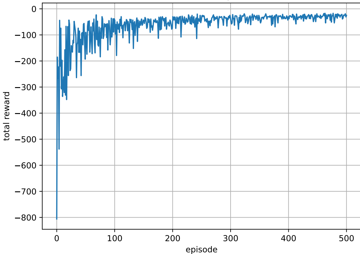
total reward vs episode
