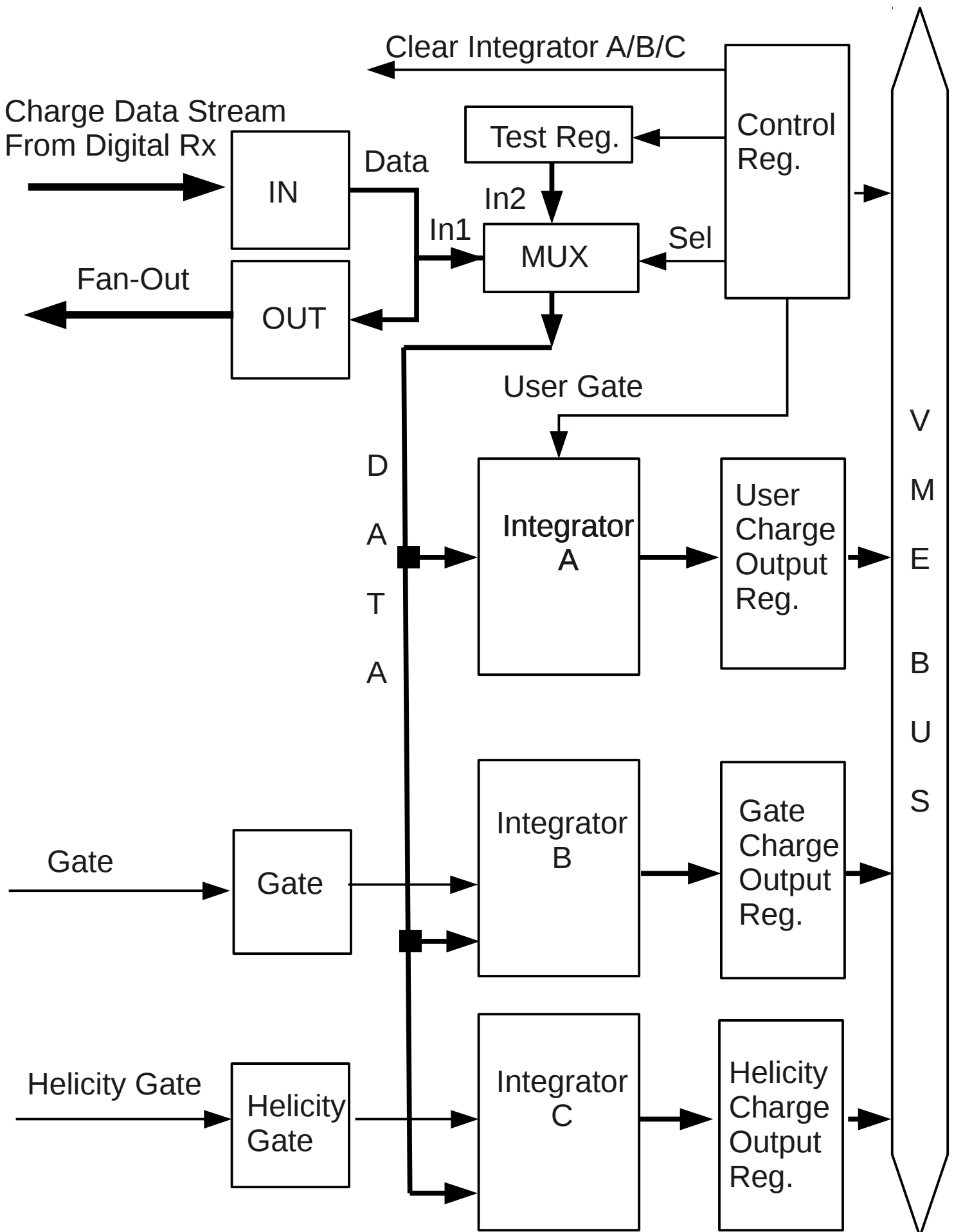
Functional Diagram of Digital Charge Readout Unit
