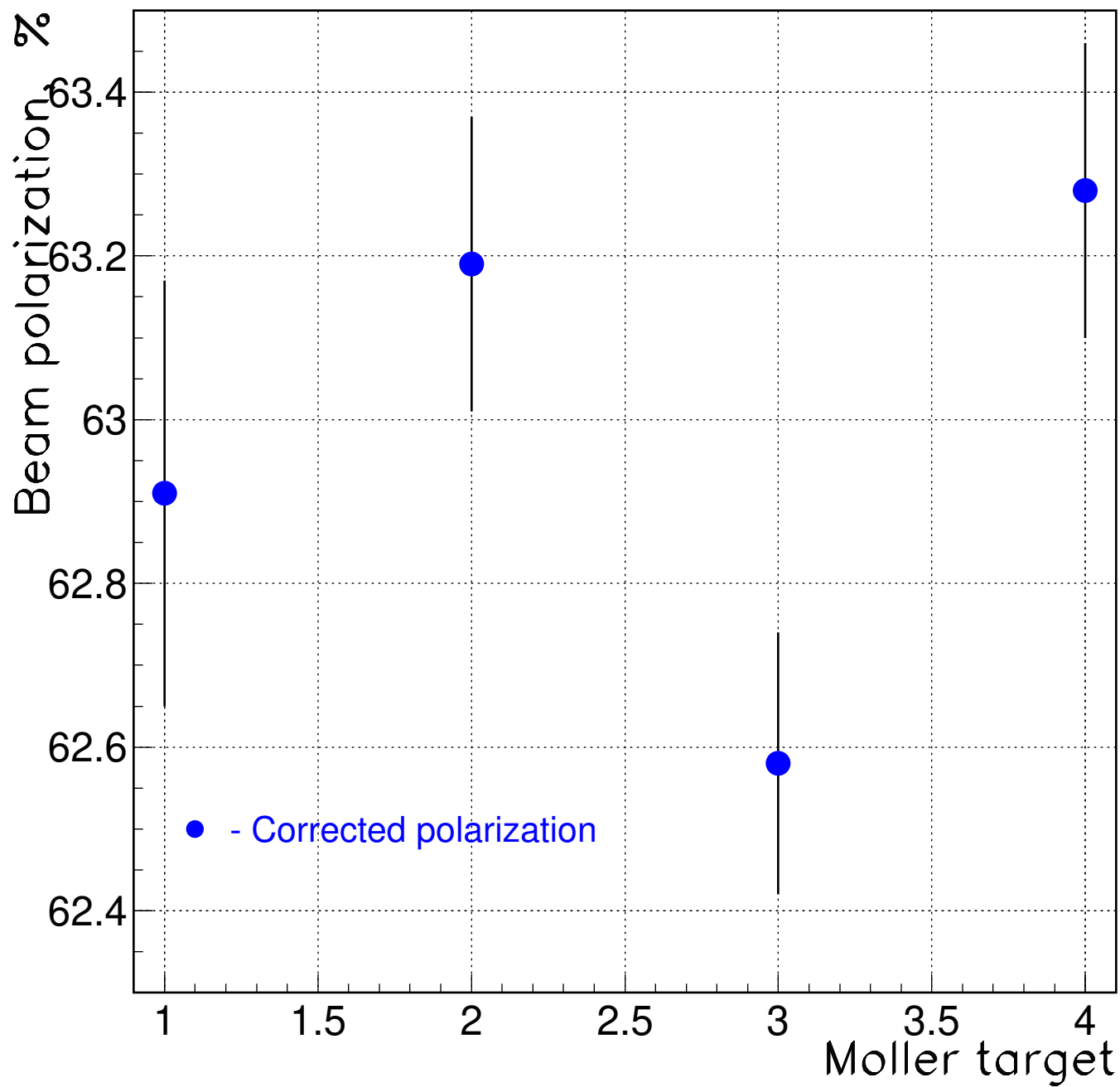
Beam Polarization vs Moller Target
