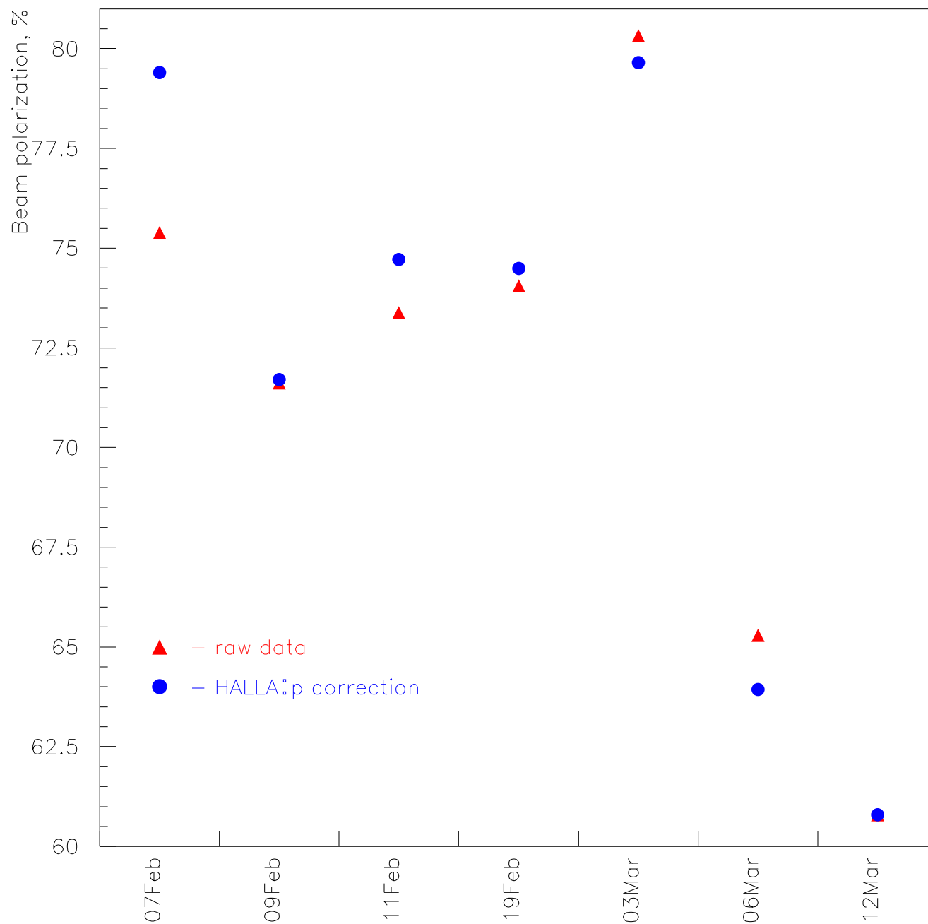
Moller measurements summary for E06-014 d2n
