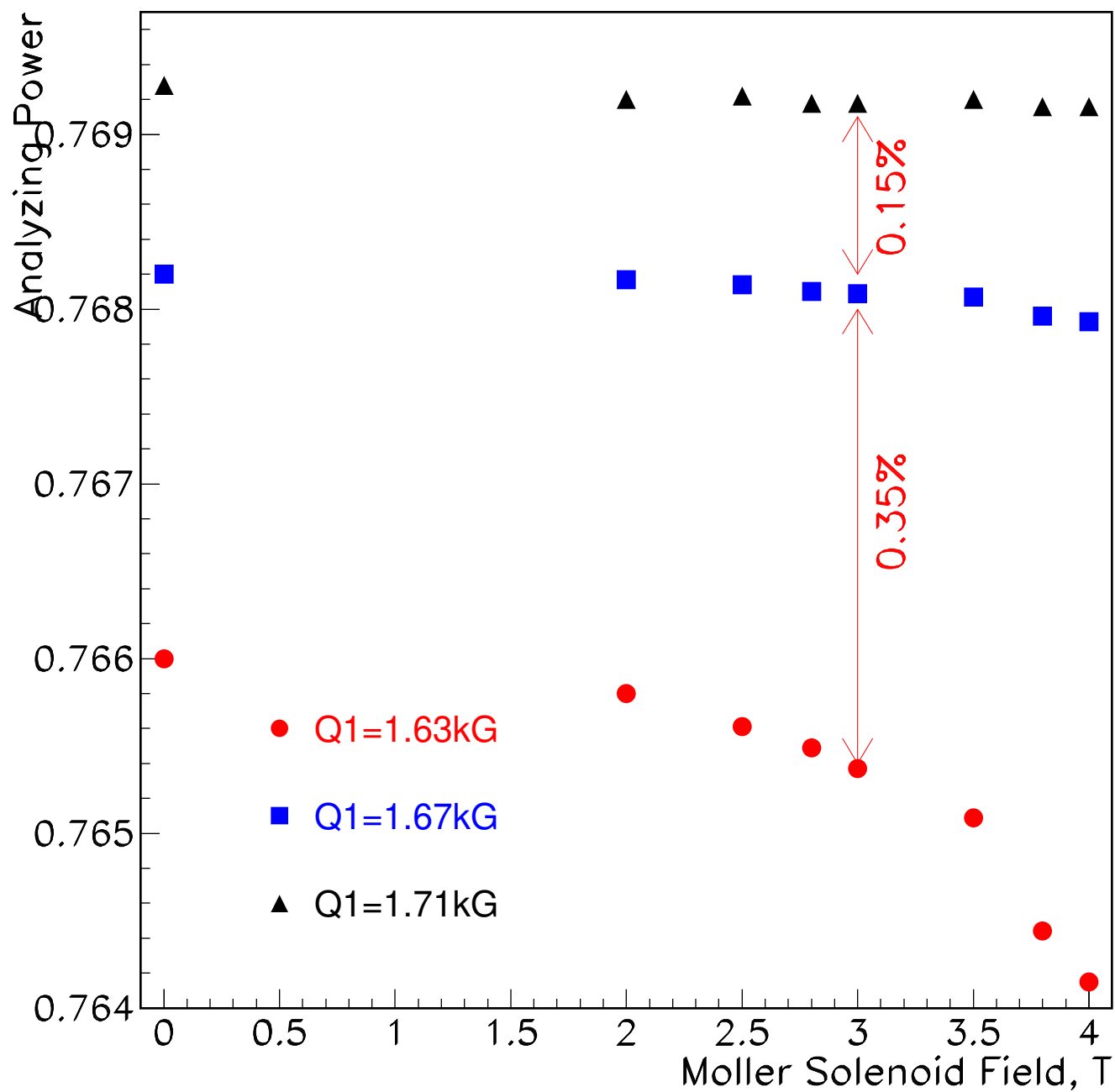
MOLLER ANALYZING POWER vs. SATURATED FIELD
