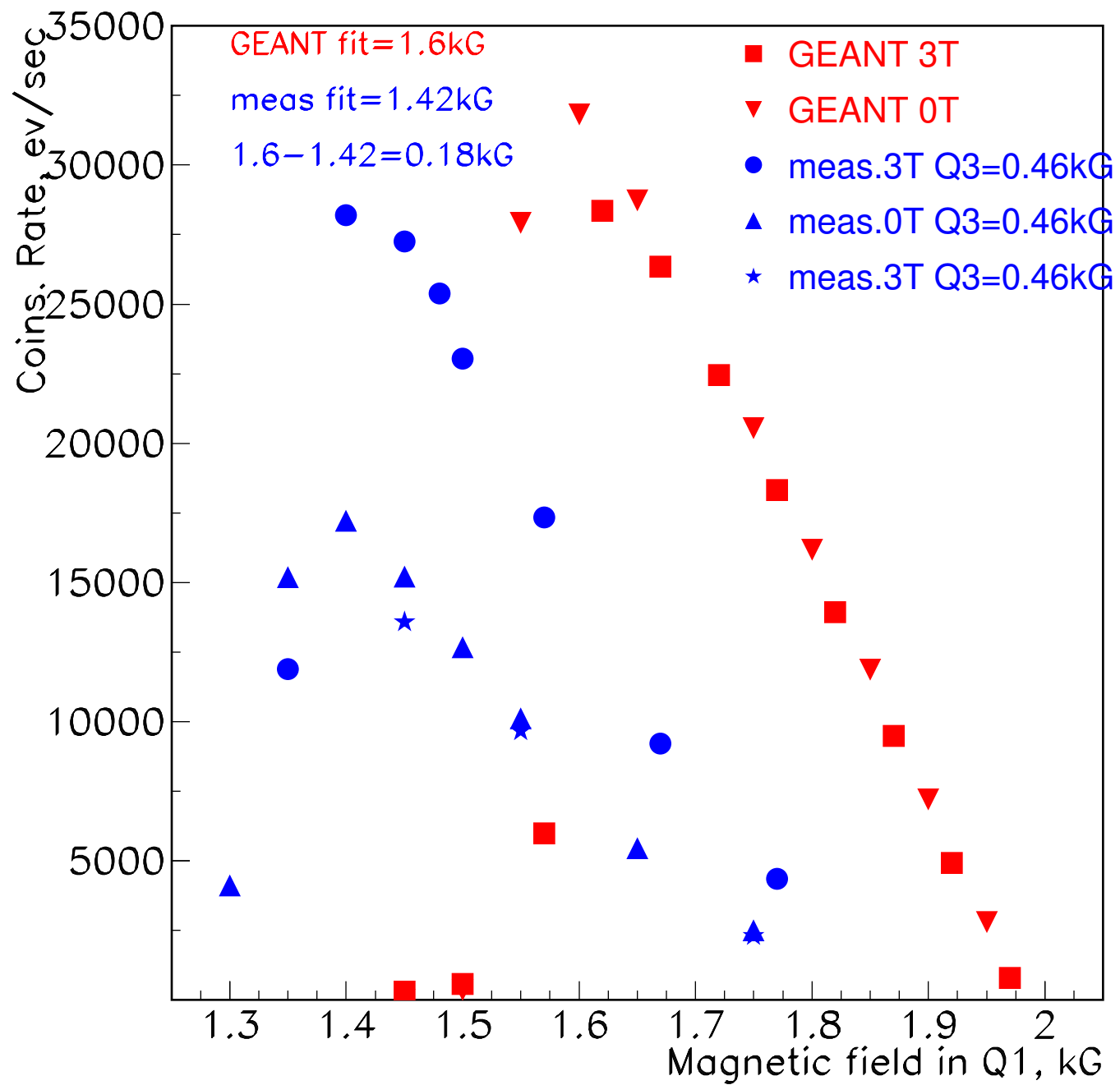
Quad Q1 Scan. Measurement vs. GEANT
