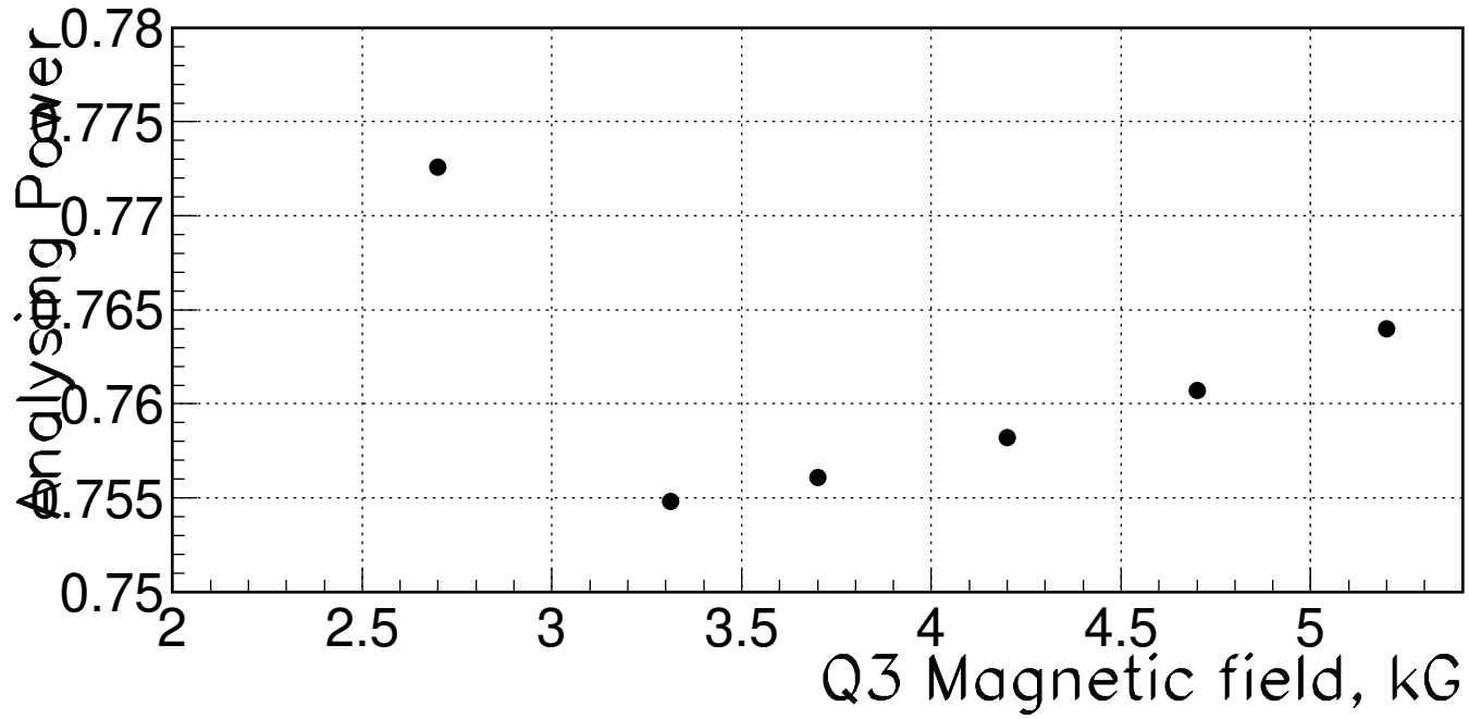
3st Moller Quad Scan
