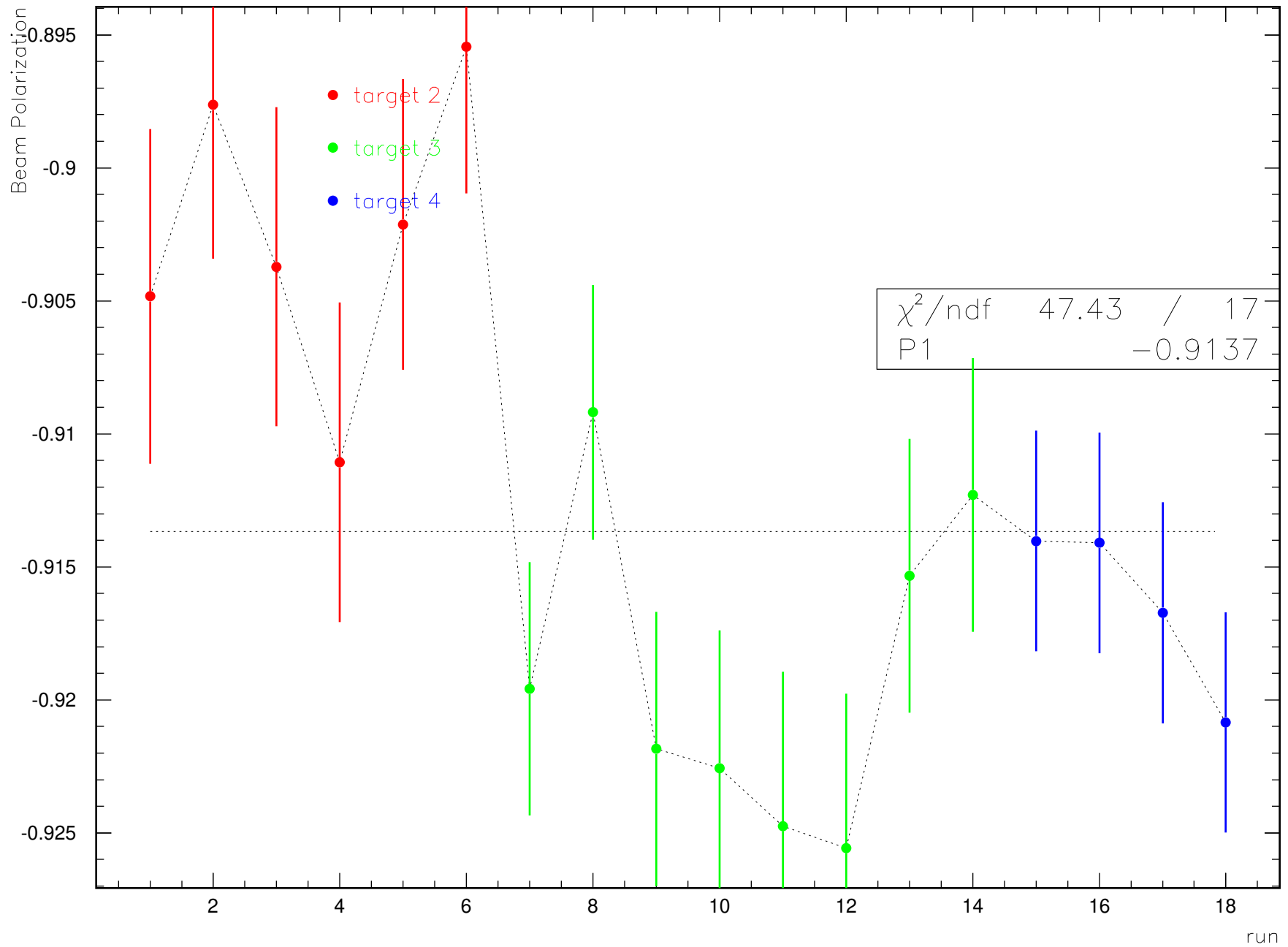
Polarization for runs 14653 – 14670
