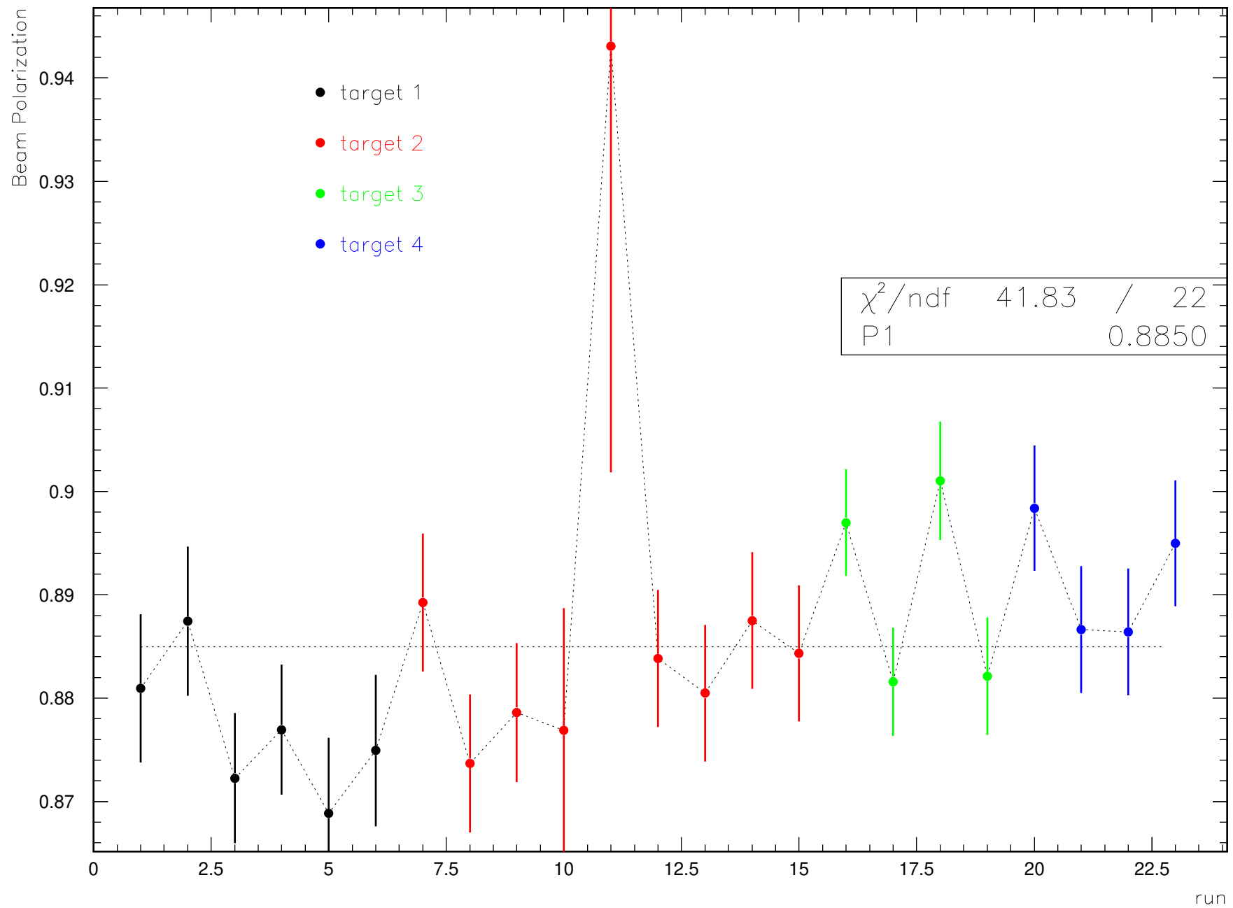
Polarization for runs 14316 – 14338
