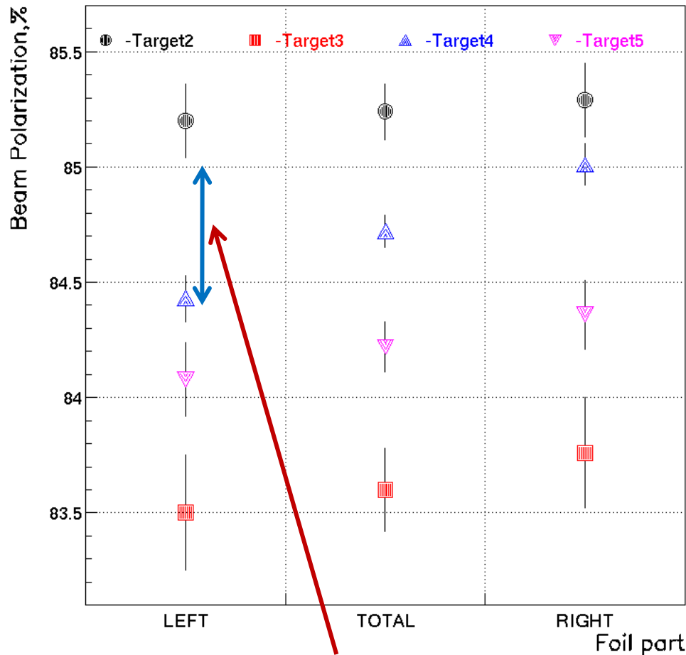
Moller Targets Double Scan Results
