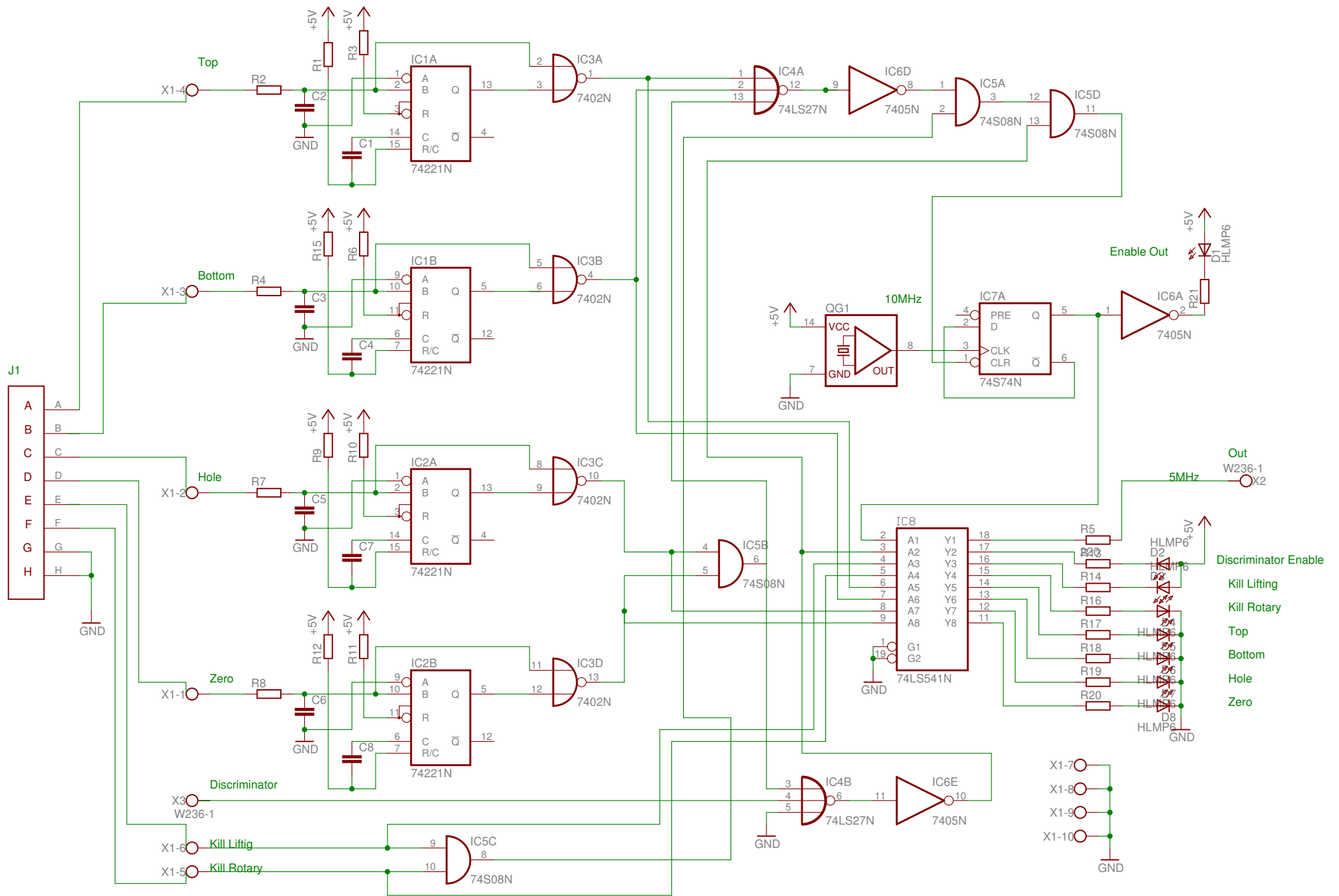
Moller Target FSD System
