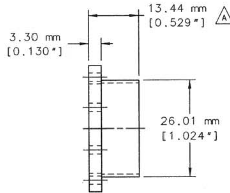
R SIDE VIEW 1-3B
