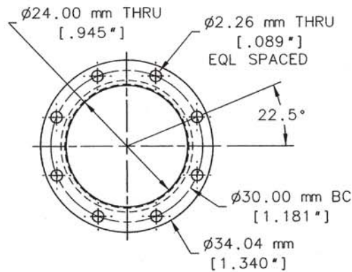
FRONT VIEW 1-4B
