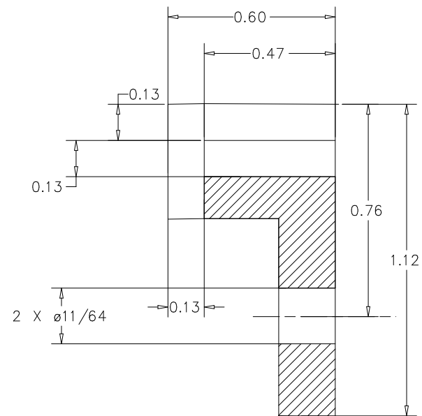
SECT 1-4B VIEW M 5:1
