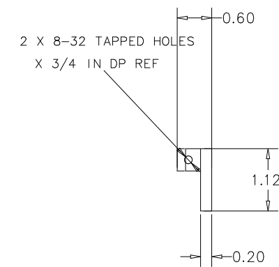
RT SIDE VIEW
